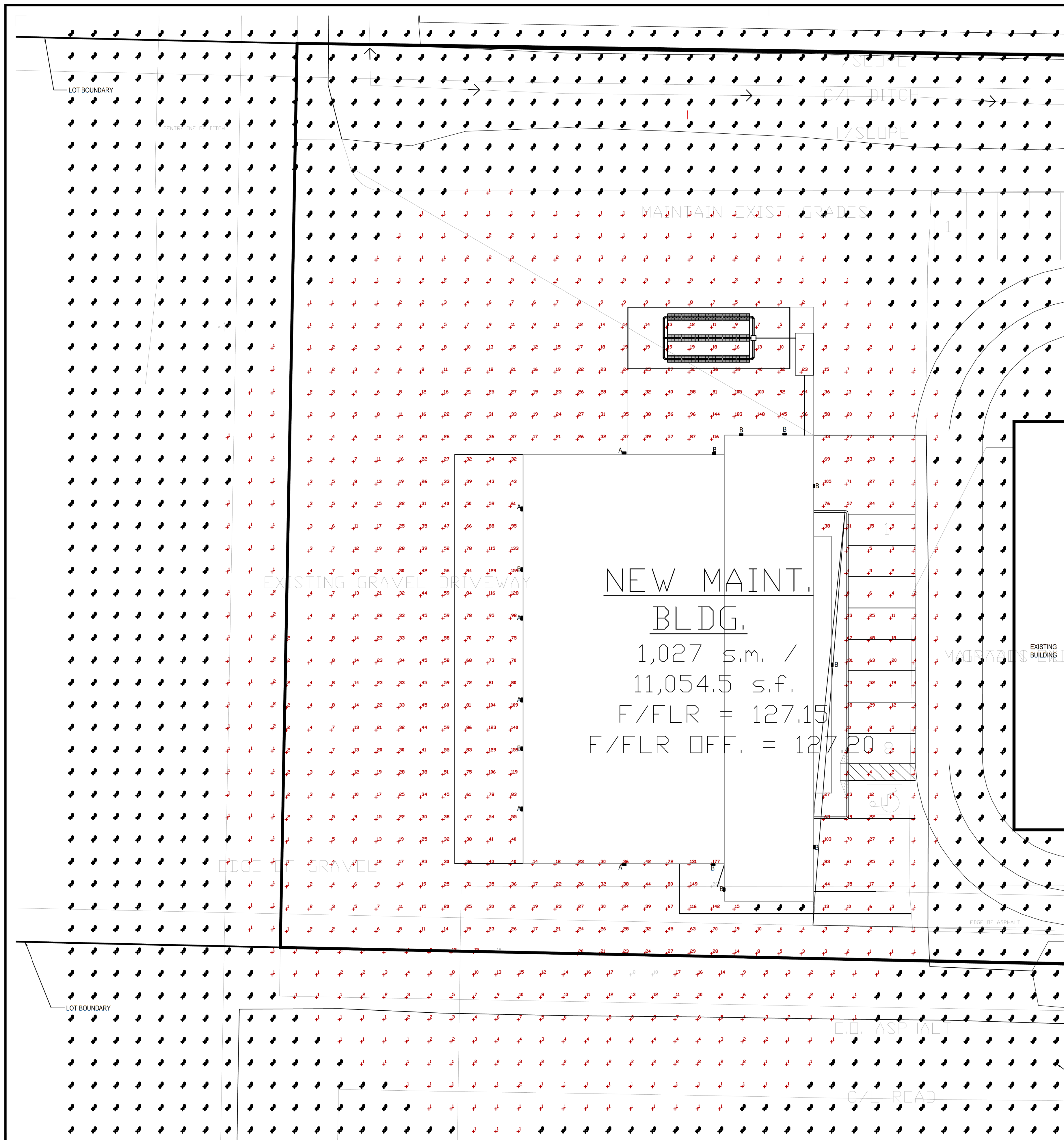
01 SITE LIGHTING PLAN 1/16"=1'
