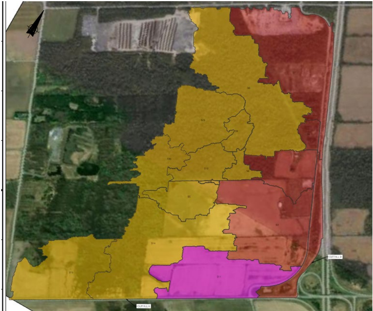
Figure 11: Pre-development sub-catchments (Drawing 7154024-200000-41-D30-0003 extract)
