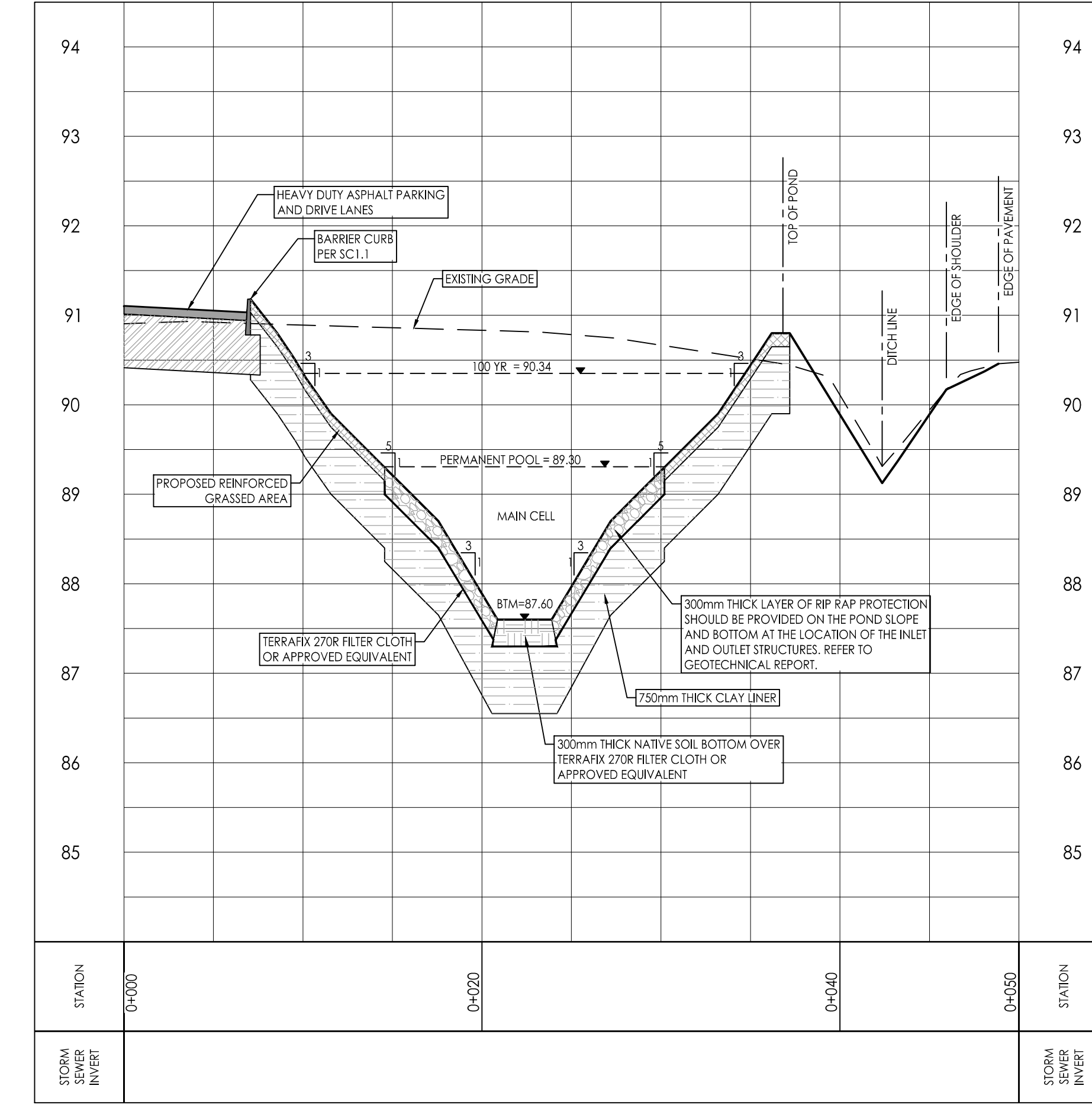
SECTION B-B MAIN CELL Scale: 1:250
