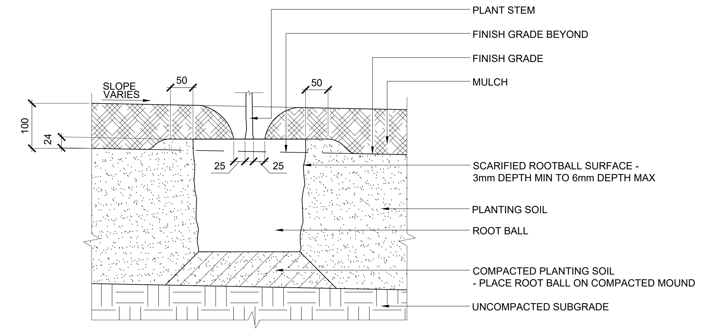
3 SHRUB PLANTING SCALE 1 : 5 SECTION
