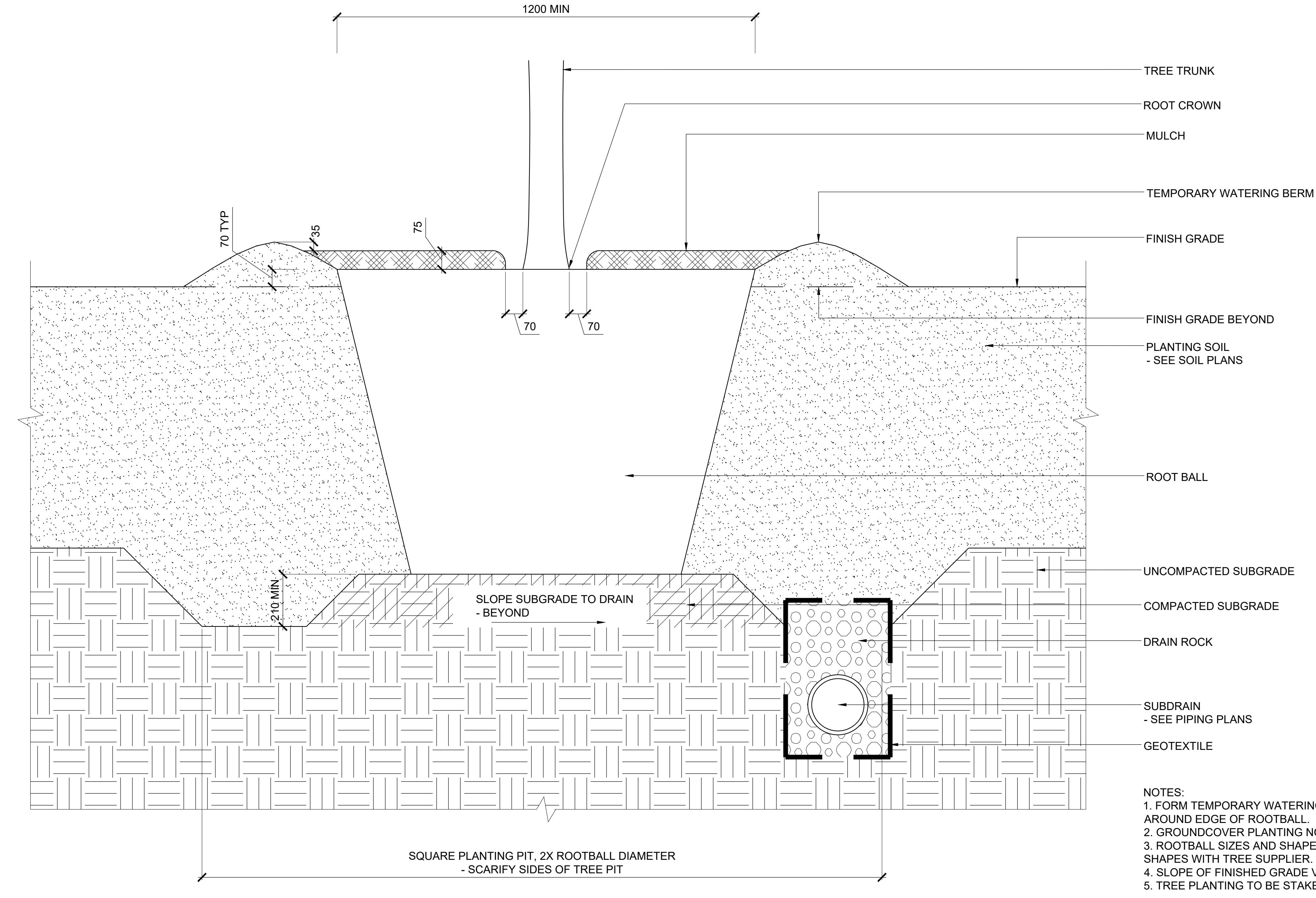
1 TREE PLANTING SCALE 1 : 10 SECTION
