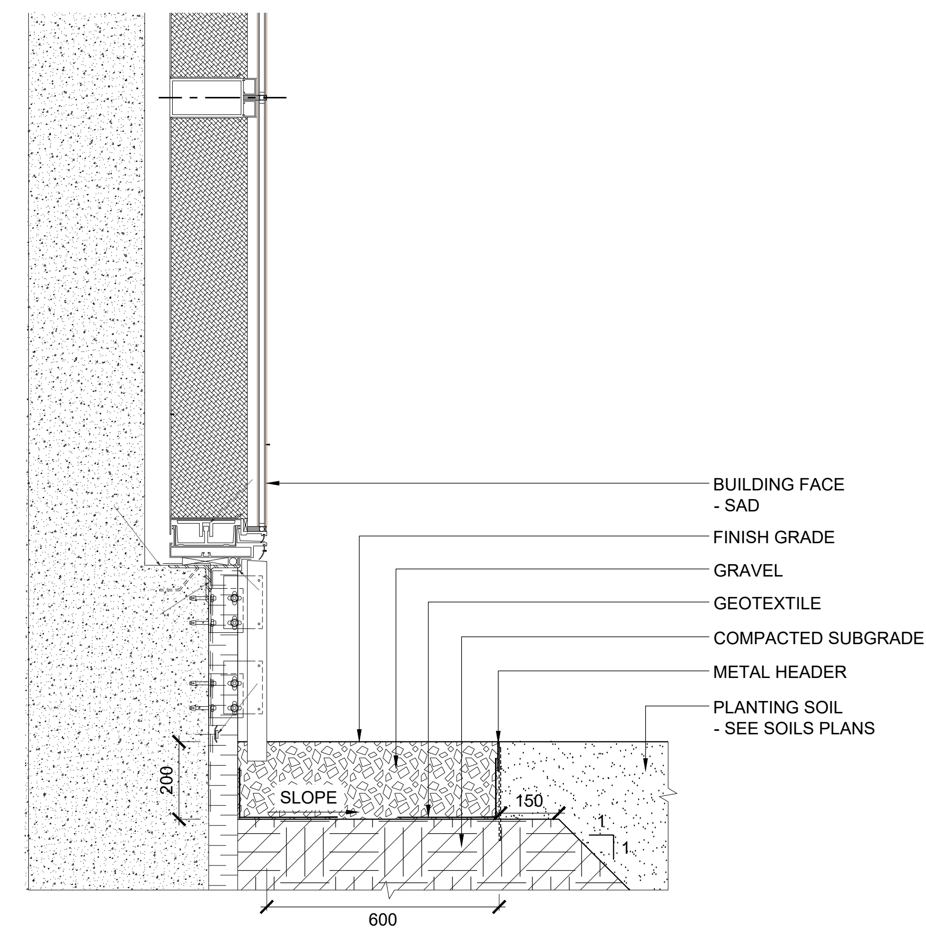
5 GRAVEL MAINTENANCE BAND AT TOWER A CW-02 SCALE 1 : 10 TYPICAL SECTION
