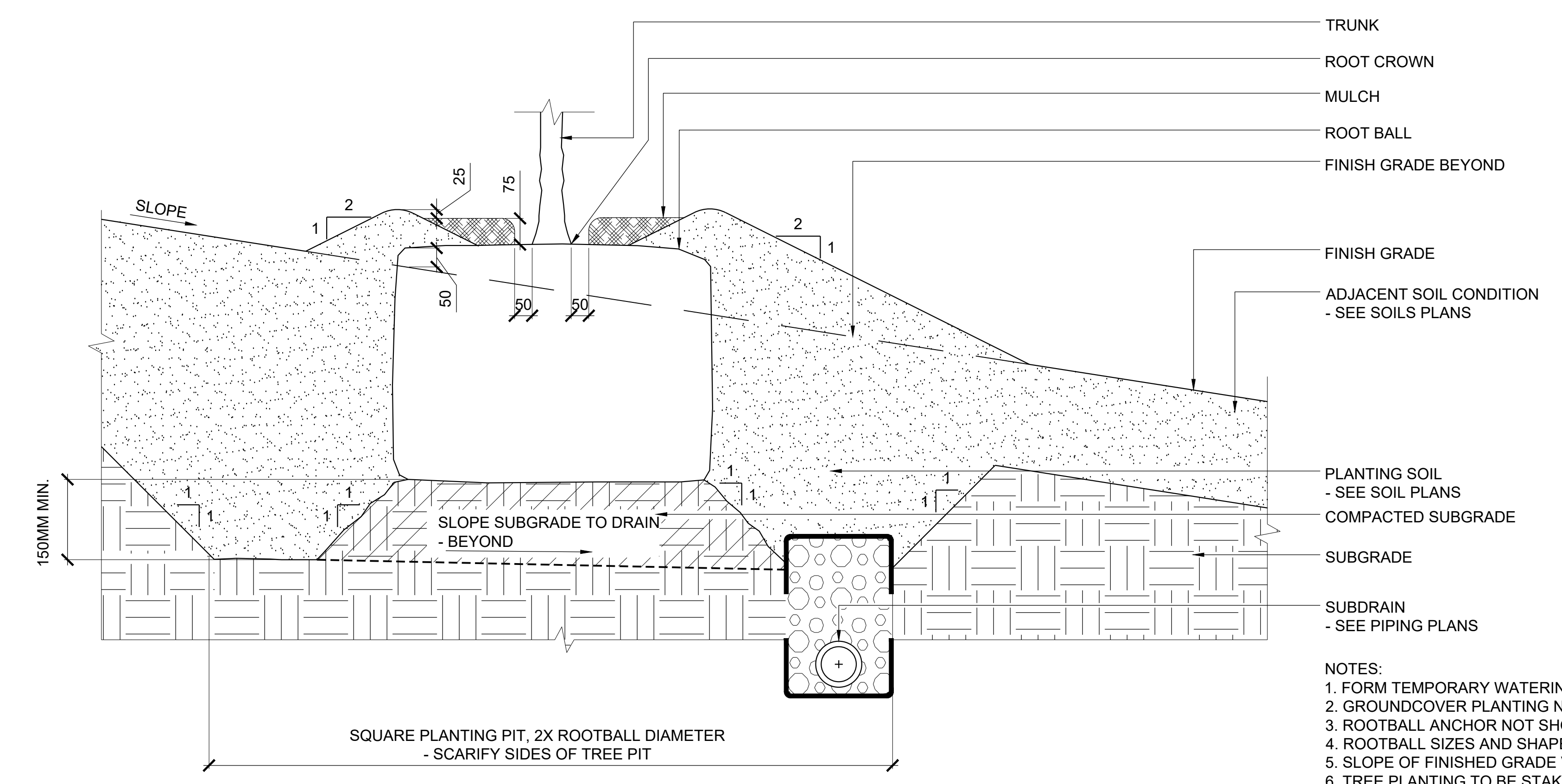
2 TREE PLANTING ON SLOPE SCALE 1 : 10 SECTION
