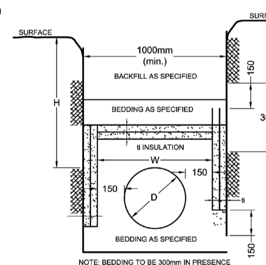
INSULATION DETAIL FOR SHALLOW SEWERS & WATERMAIN
