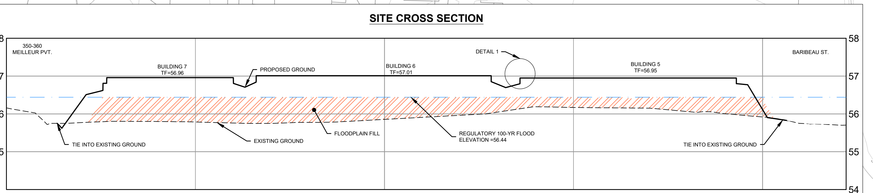
SECTION A-A HORIZONTAL SCALE 1:300 VERTICAL SCALE 1:60
