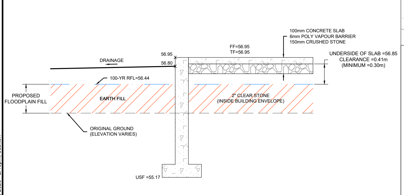
DETAIL 1 - BUILDING 5: FLOOD PROOFING N.T.S.
