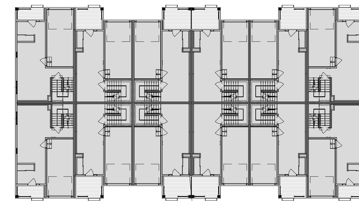
BUILDING AREA 700 m 2
