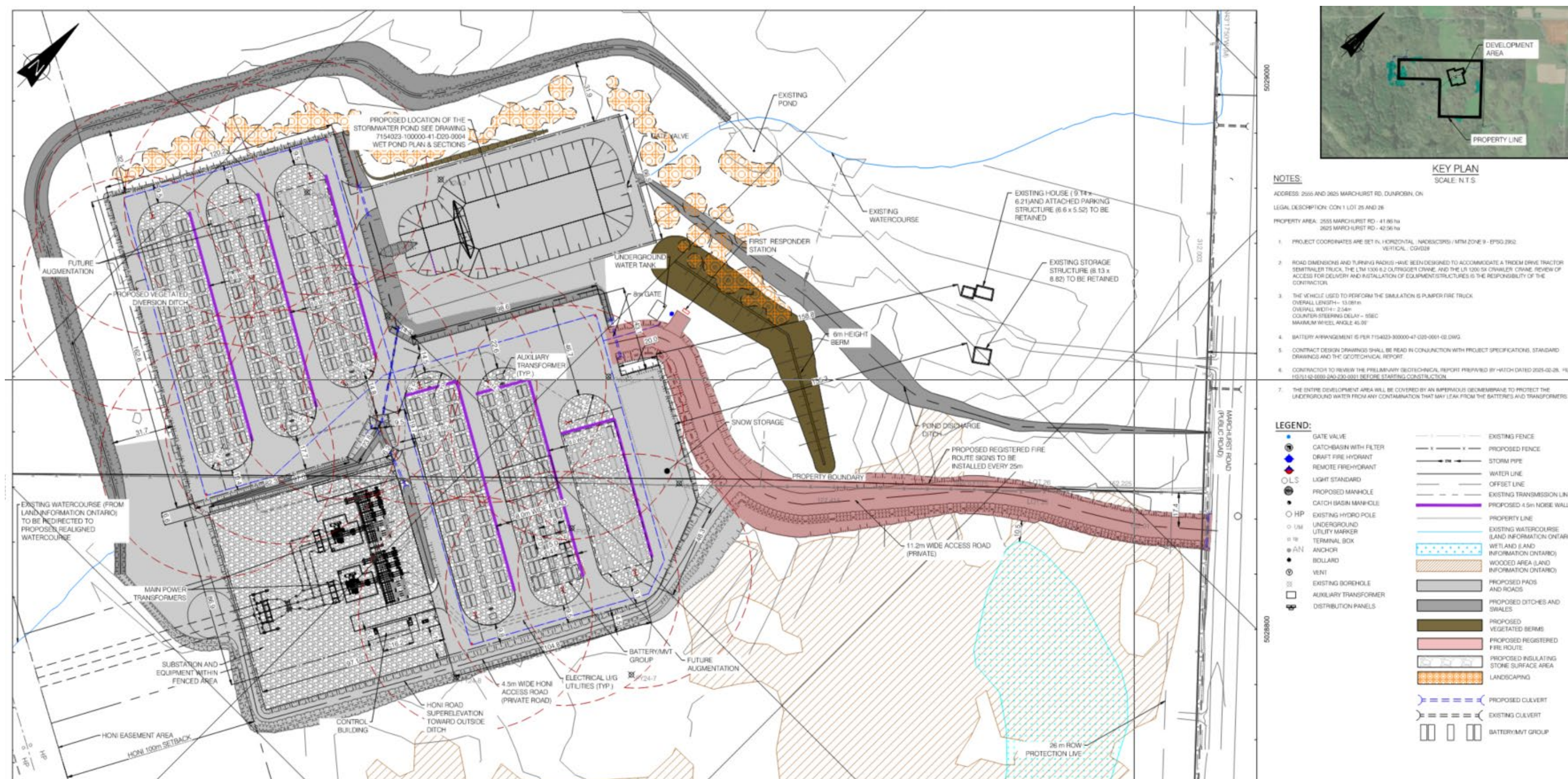
Figure 3: Watercourse path through the BESS site
