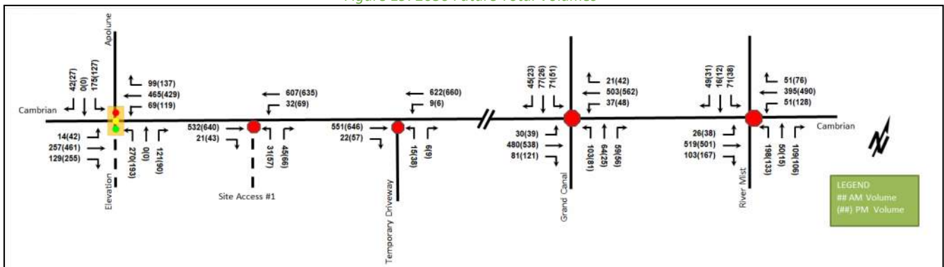
Figure 19: 2030 Future Total Volumes
