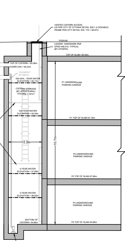
CISTERN #1 DETAIL
