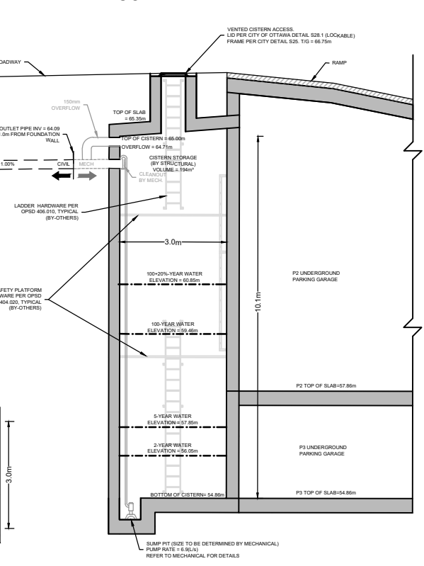
CISTERN #2 DETAIL
