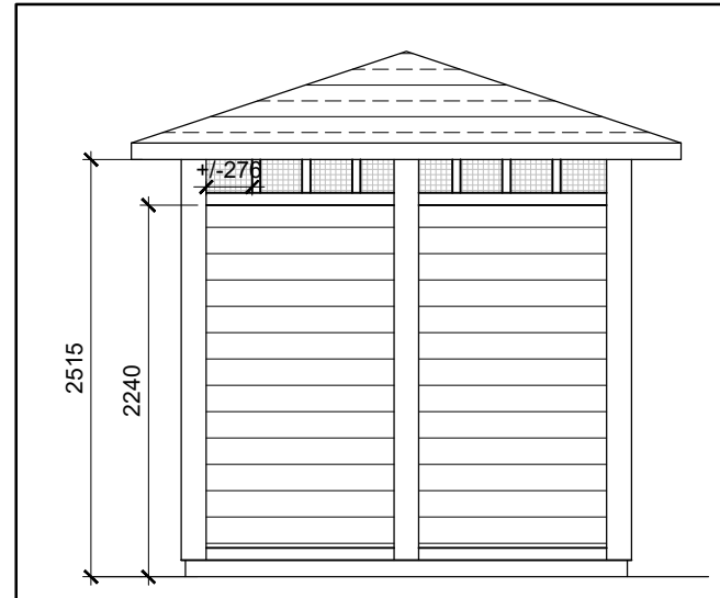
3 GARBAGE ENCLOSURE A-100 REAR ELEVATION SCALE = 1 : 50
