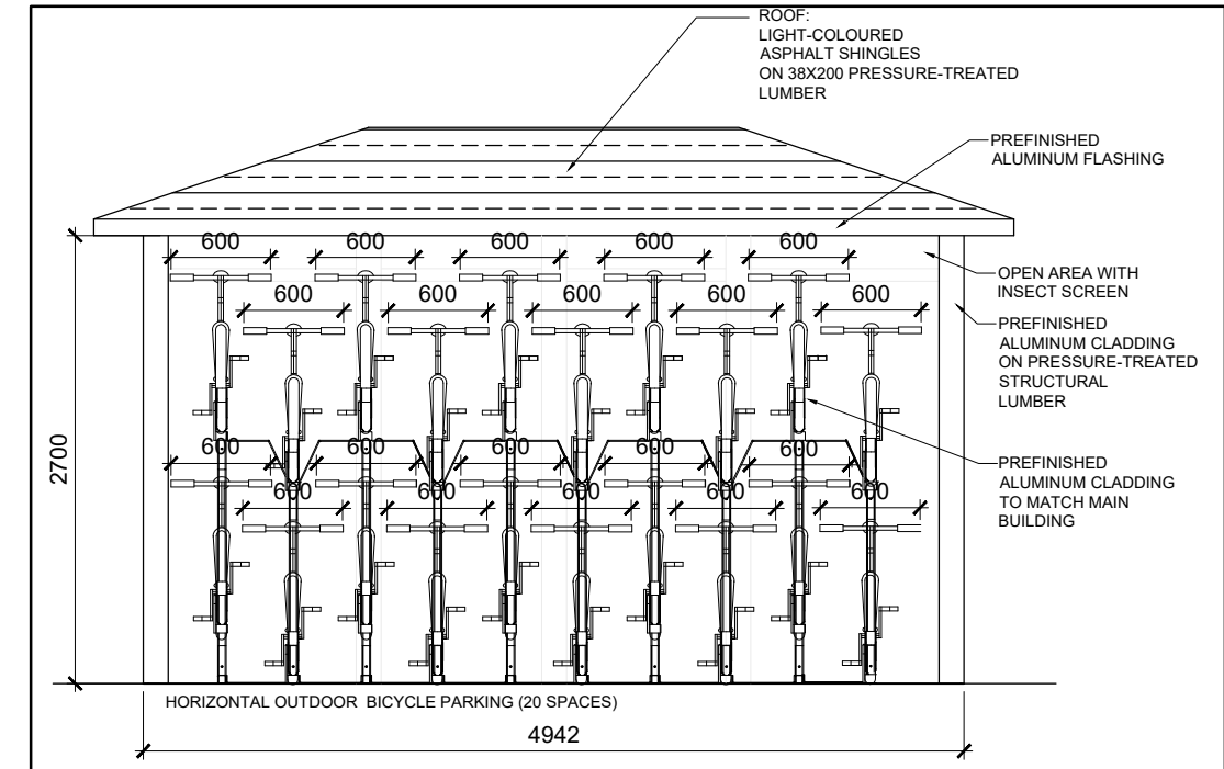
7 BICYCLE PARKING INTERIOR ELEVATION A-100 SCALE = 1 : 50
