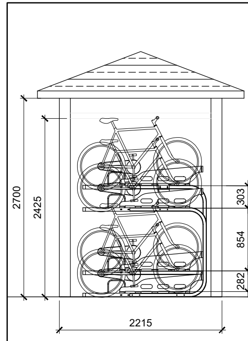
8 BICYCLE PARKING CROSS SECTION A-100 SCALE = 1 : 50
