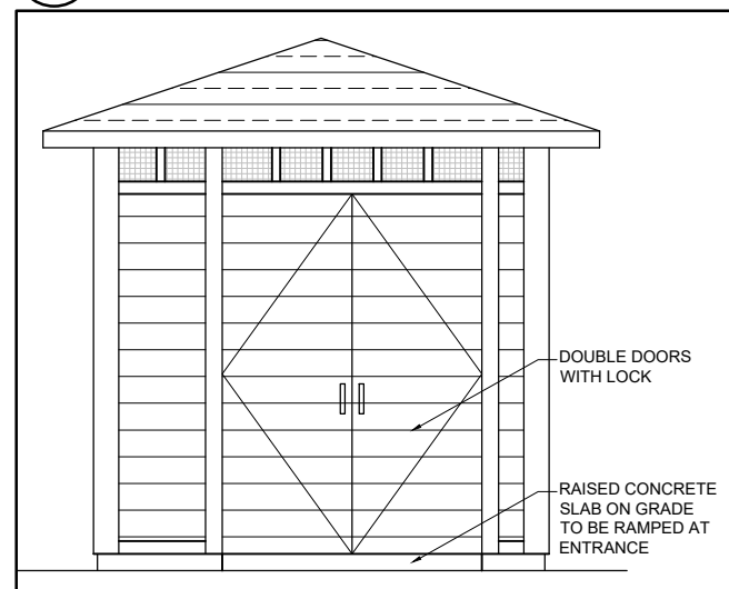
4 GARBAGE ENCLOSURE A-100 FRONT ELEVATION SCALE = 1 : 50
