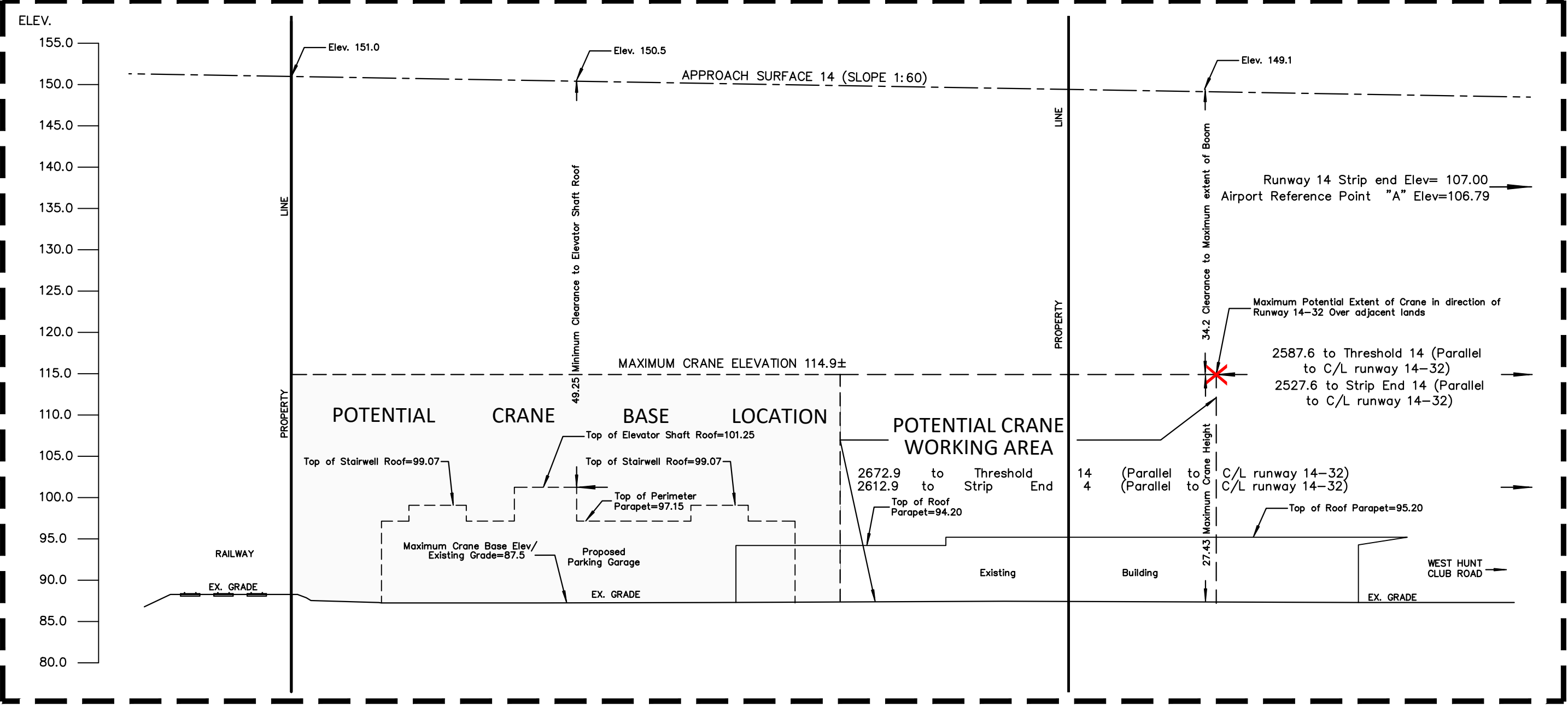
SECTION A-A (Parallel to Runway 14-32) Scale 1: 500
