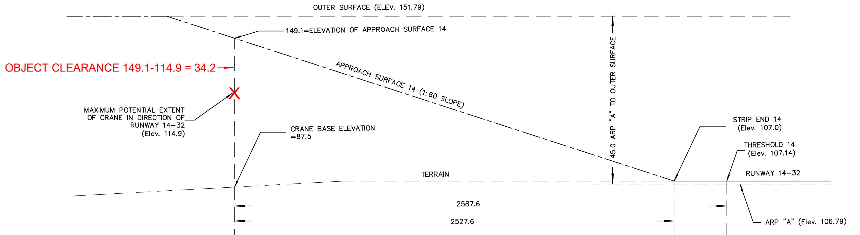
Section along Approach Surface (Not to Scale)
