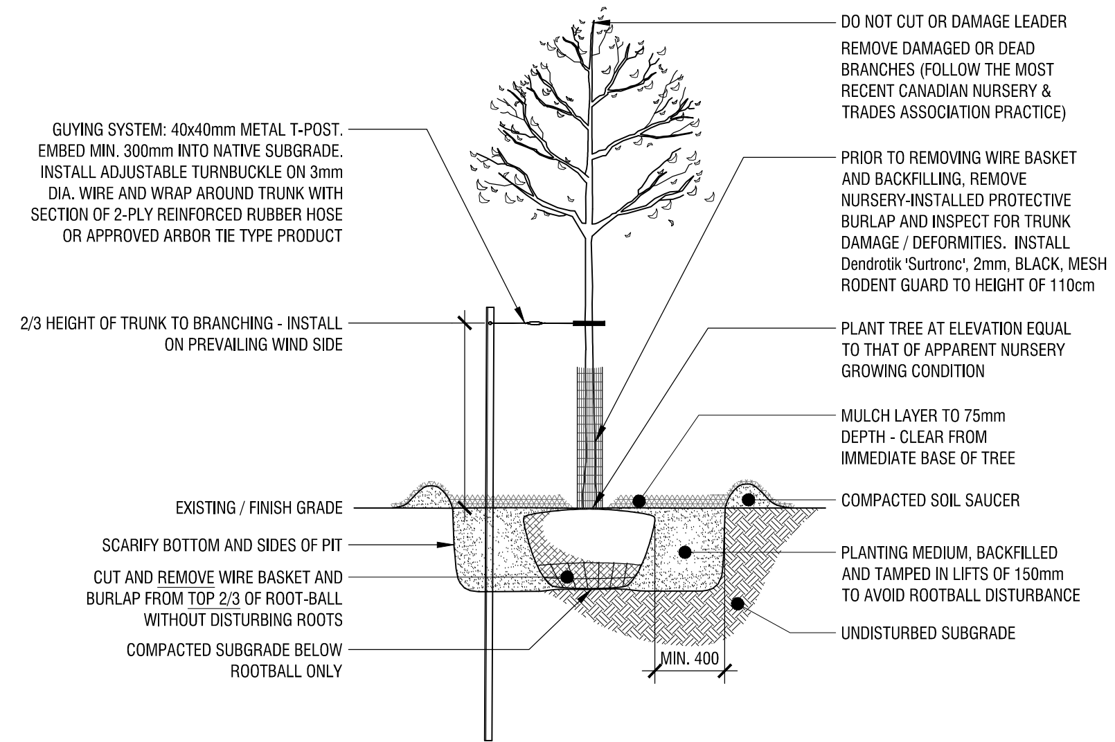
1 DECIDUOUS PLANTING DETAIL L7 N.T.S.
