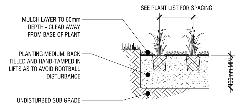
4 PERENNIAL PLANTING DETAIL L7 N.T.S.
