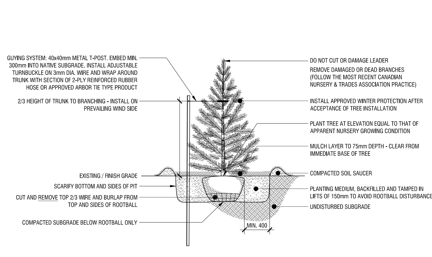
2 CONIFEROUS PLANTING DETAIL L7 N.T.S.
