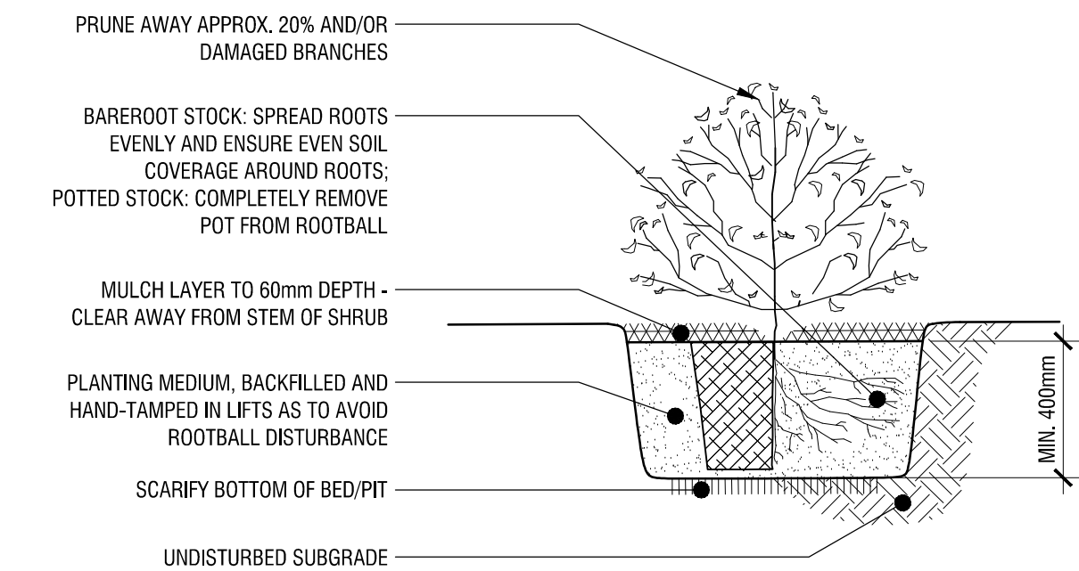
3 SHRUB PLANTING DETAIL L7 N.T.S.
