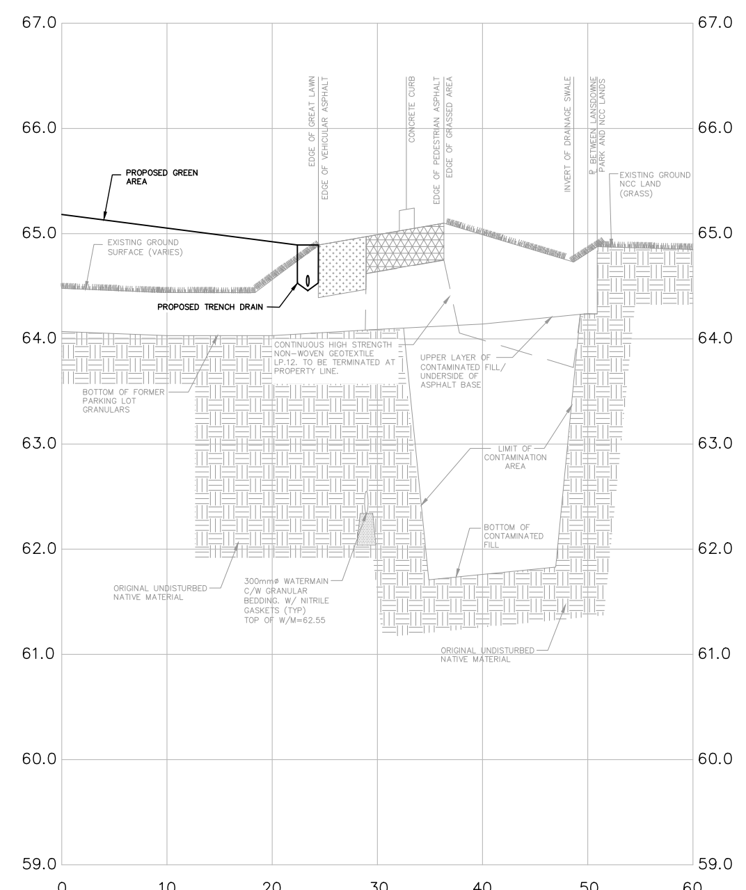
F CONTAMINATION ZONE FOR McElroy SITE CROSS SECTION F SCALE: H 1:300, V 1:30
