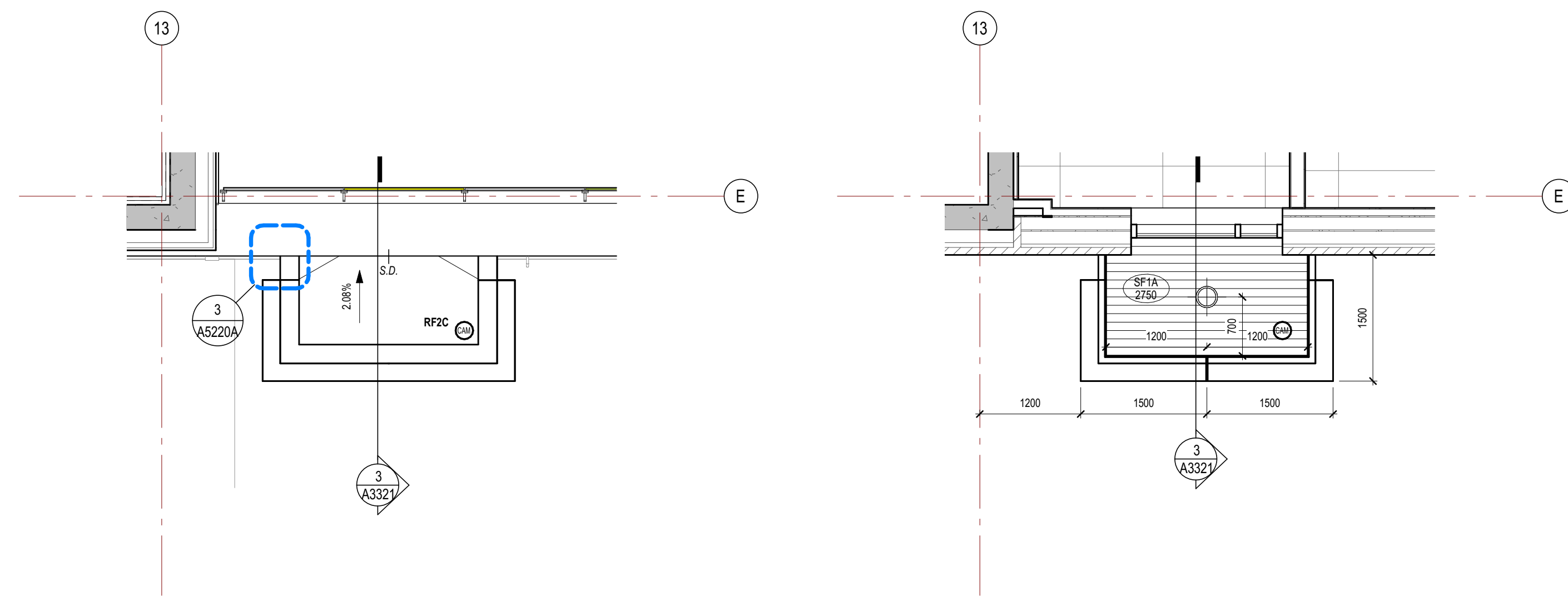
6 L1 STAFF ENTRANCE CANOPY - ROOF PLAN A1801 1:50
