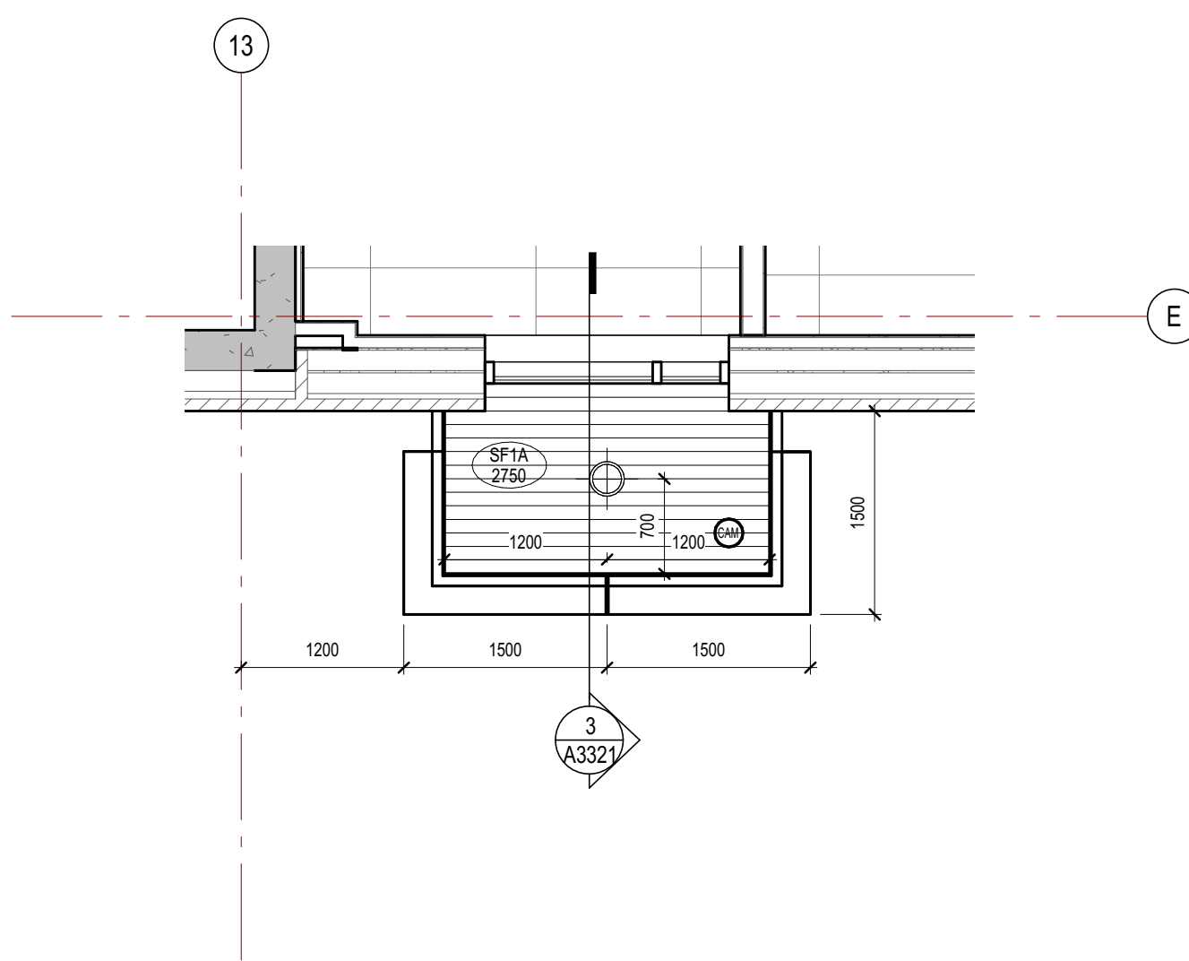
5 L1 STAFF ENTRANCE CANOPY - RCP A1801 1:50
