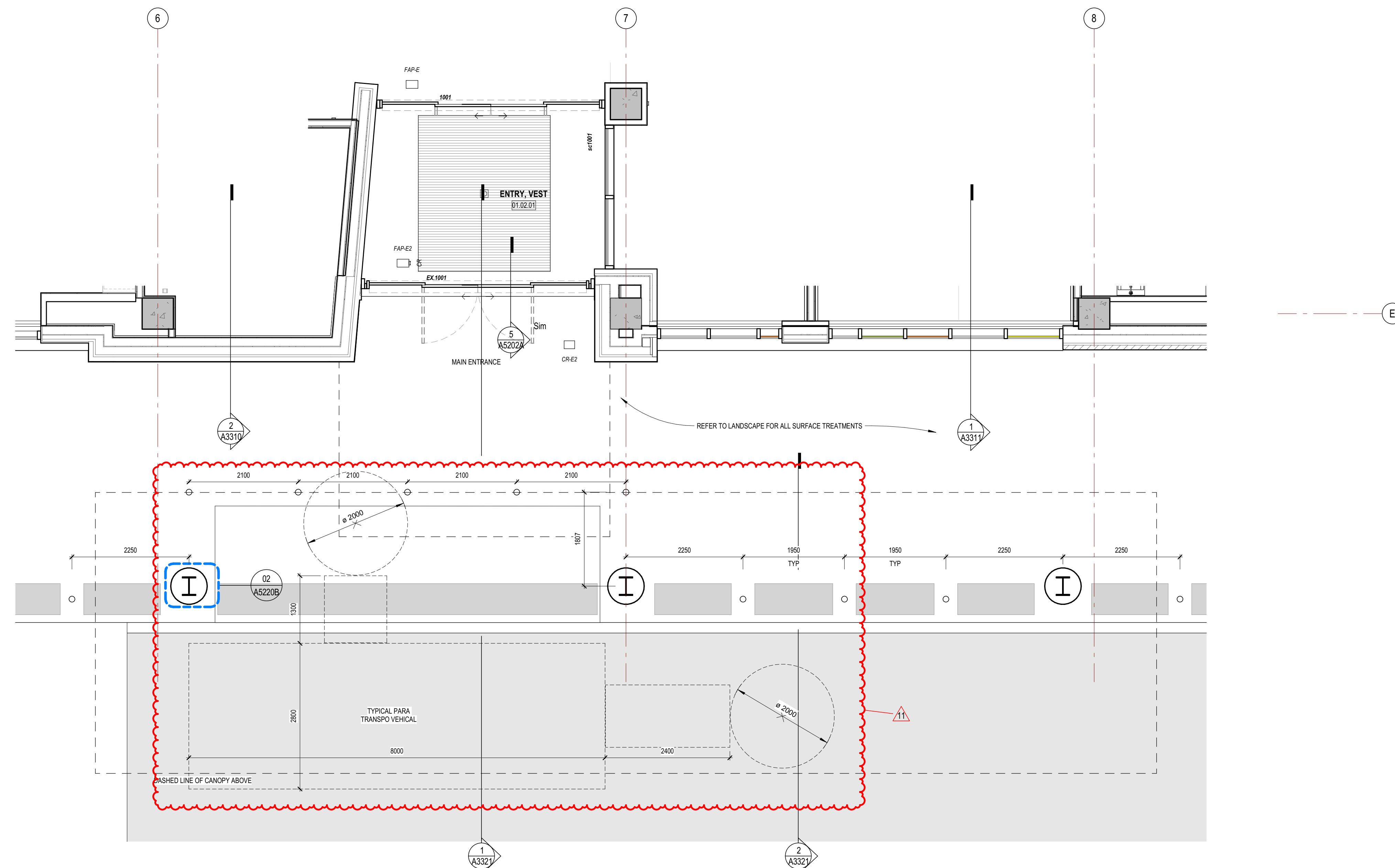
1 L1 MAIN CANOPY - PLAN A1801 1:50
