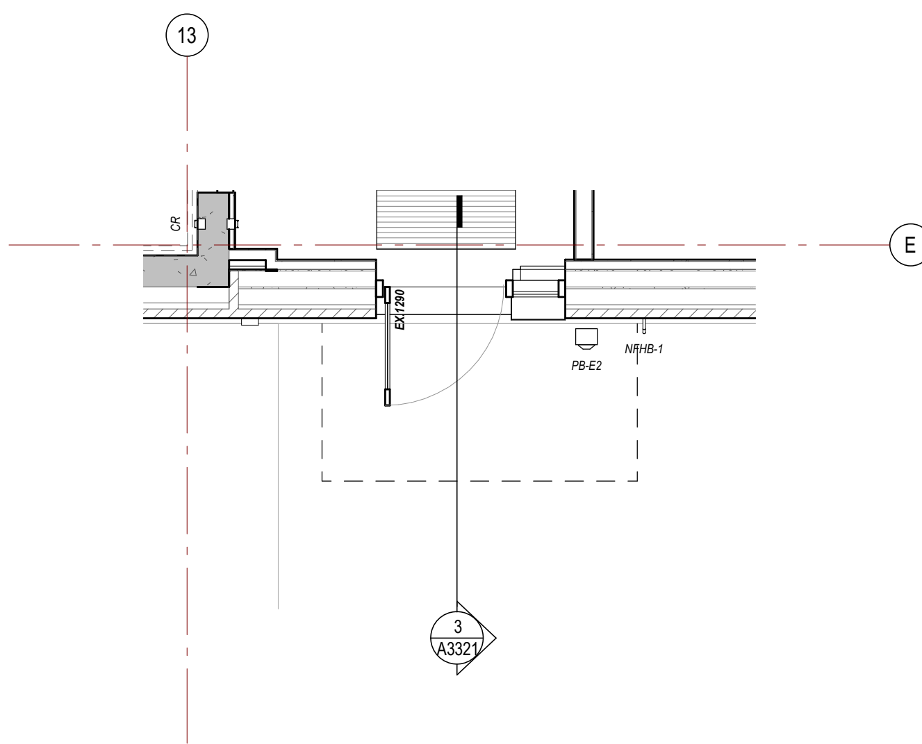
4 L1 STAFF ENTRANCE CANOPY - PLAN A1801 1:50
