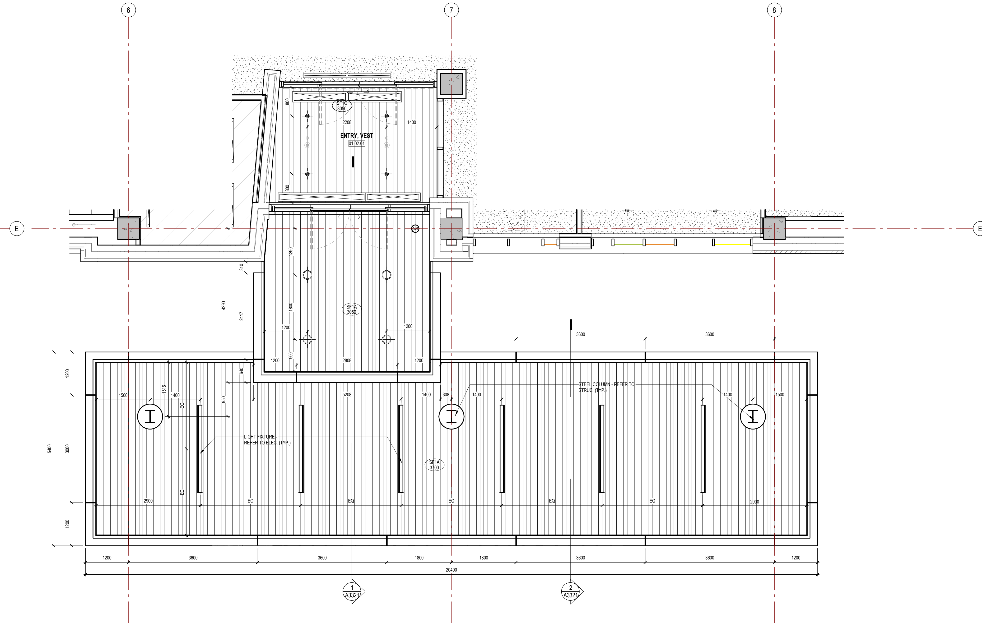
2 L1 MAIN CANOPY - RCP A1801 1:50
