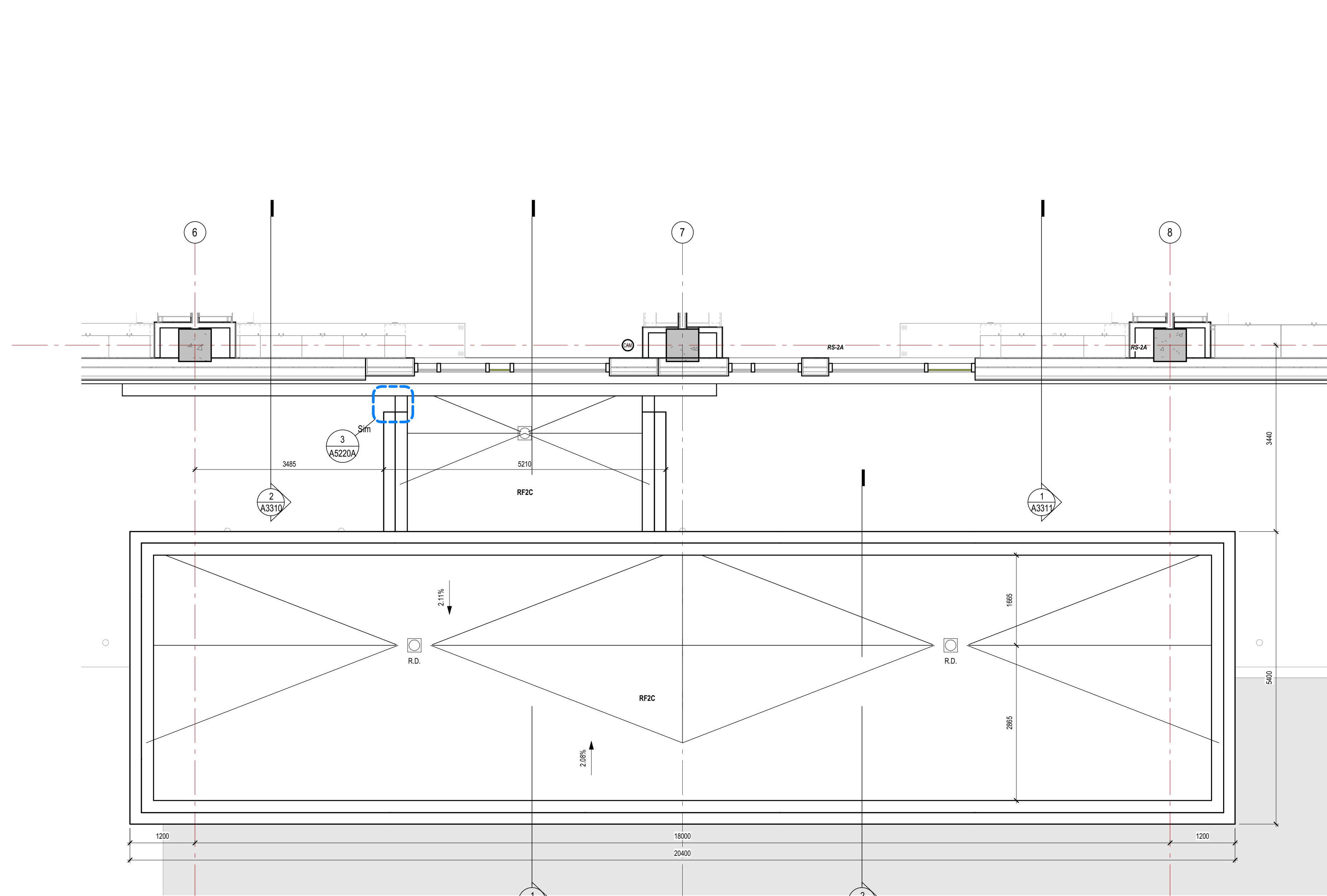
3 L1 MAIN CANOPY - ROOF PLAN A1801 1:50
