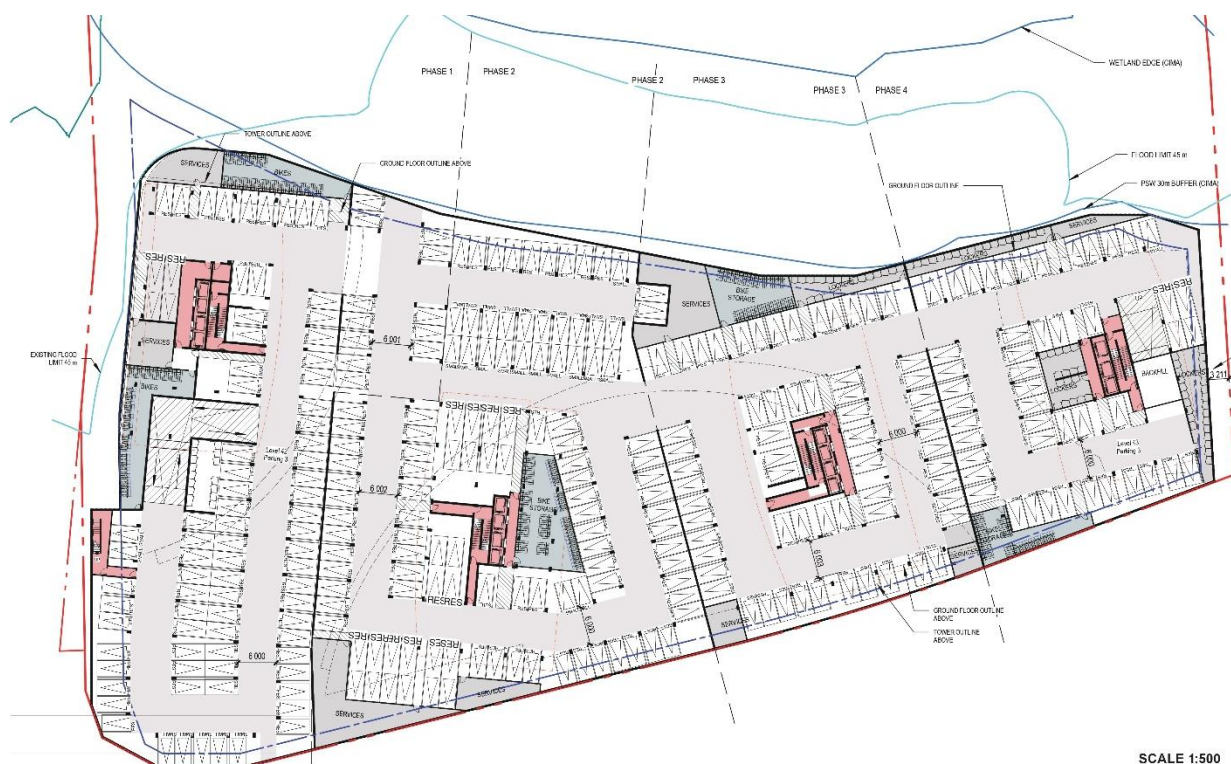
Figure 17: P3 Parking Plan (NEUF Architects)
