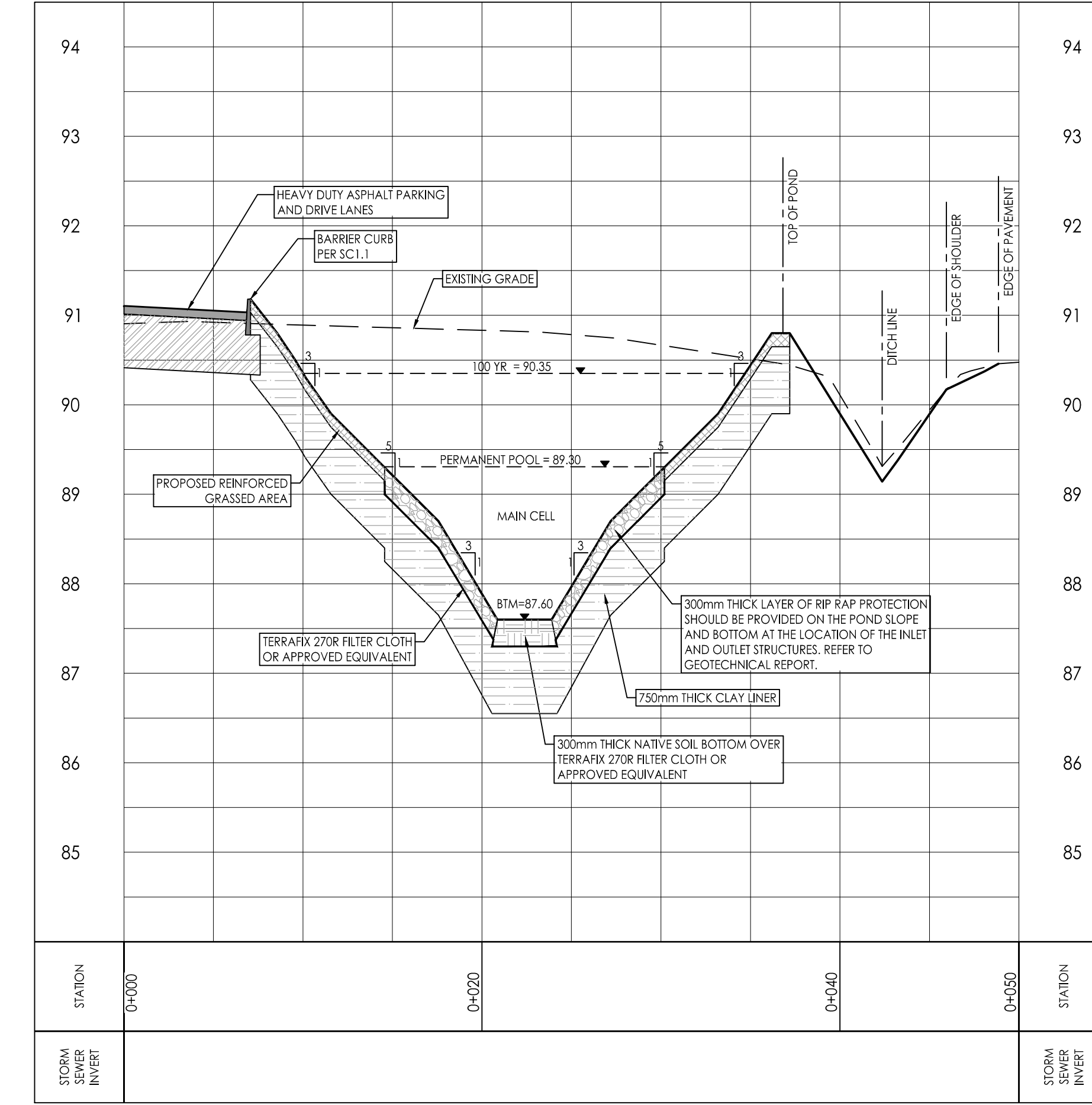
SECTION B-B MAIN CELL 1:250
