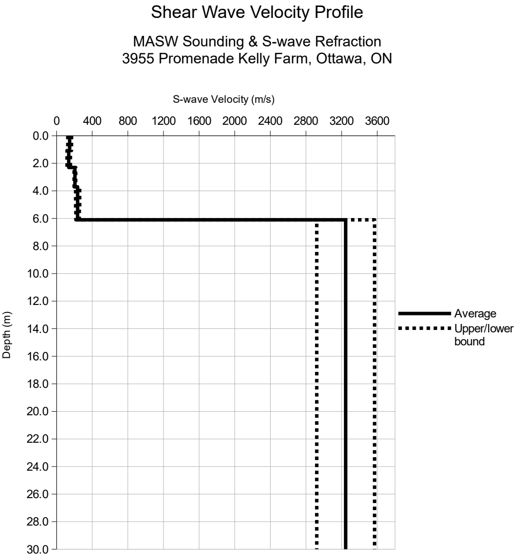
Figure 6 Shear wave velocity profile from MASW sounding and S-wave refraction.
