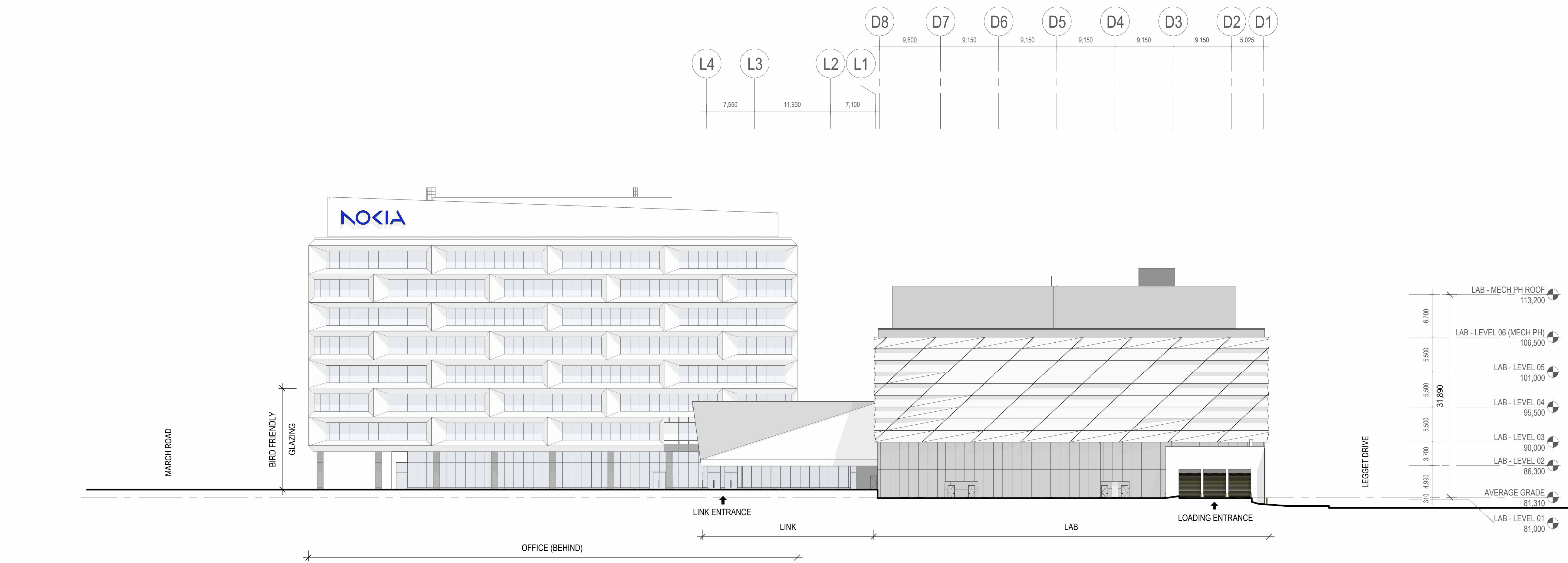
1 OVERALL BUILDING ELEVATION - SOUTH EAST SCALE: NTS
