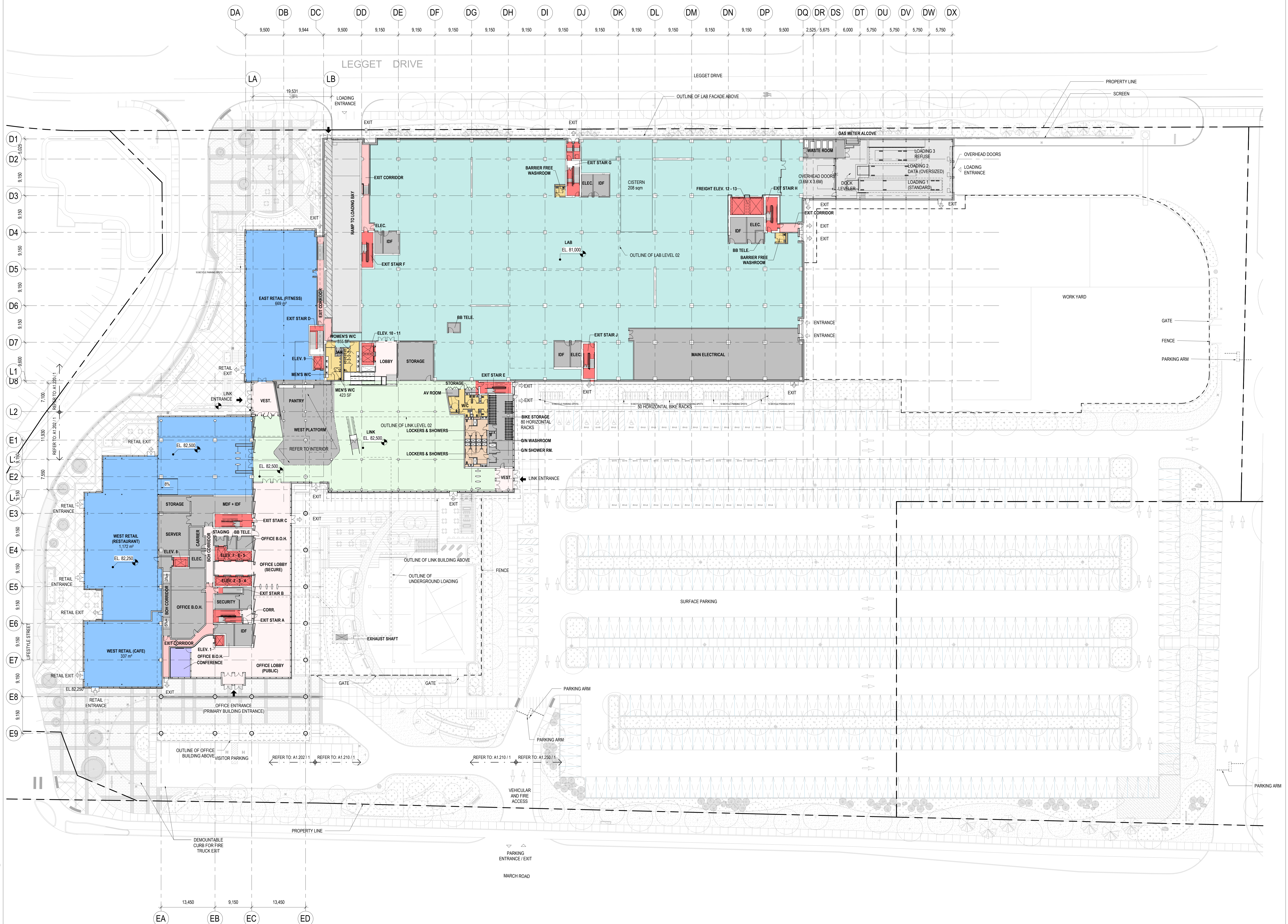
1 CONSTRUCTION PLAN - OFFICE LEVEL 01 / LAB LEVEL 01 / LINK LEVEL 01 SCALE: 1 : 300
