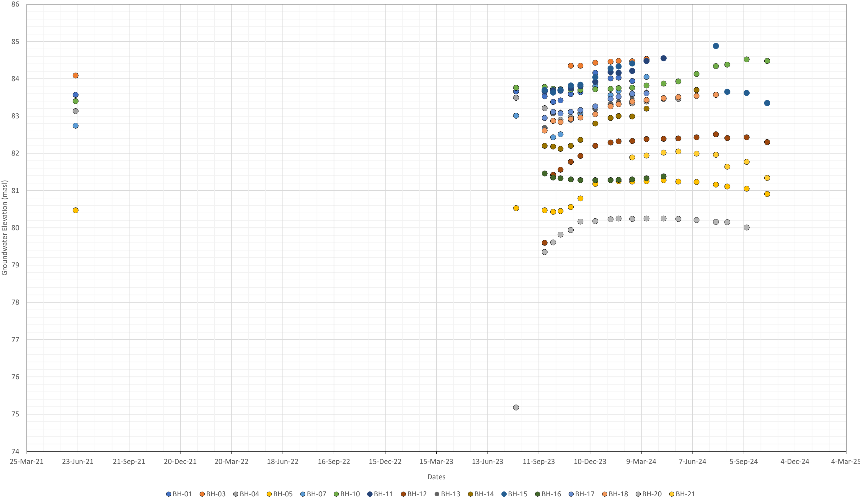
2983 Navan Road Site - Monitored Manual Groundwater Elevation Plot from June, 2021 to October,2024
