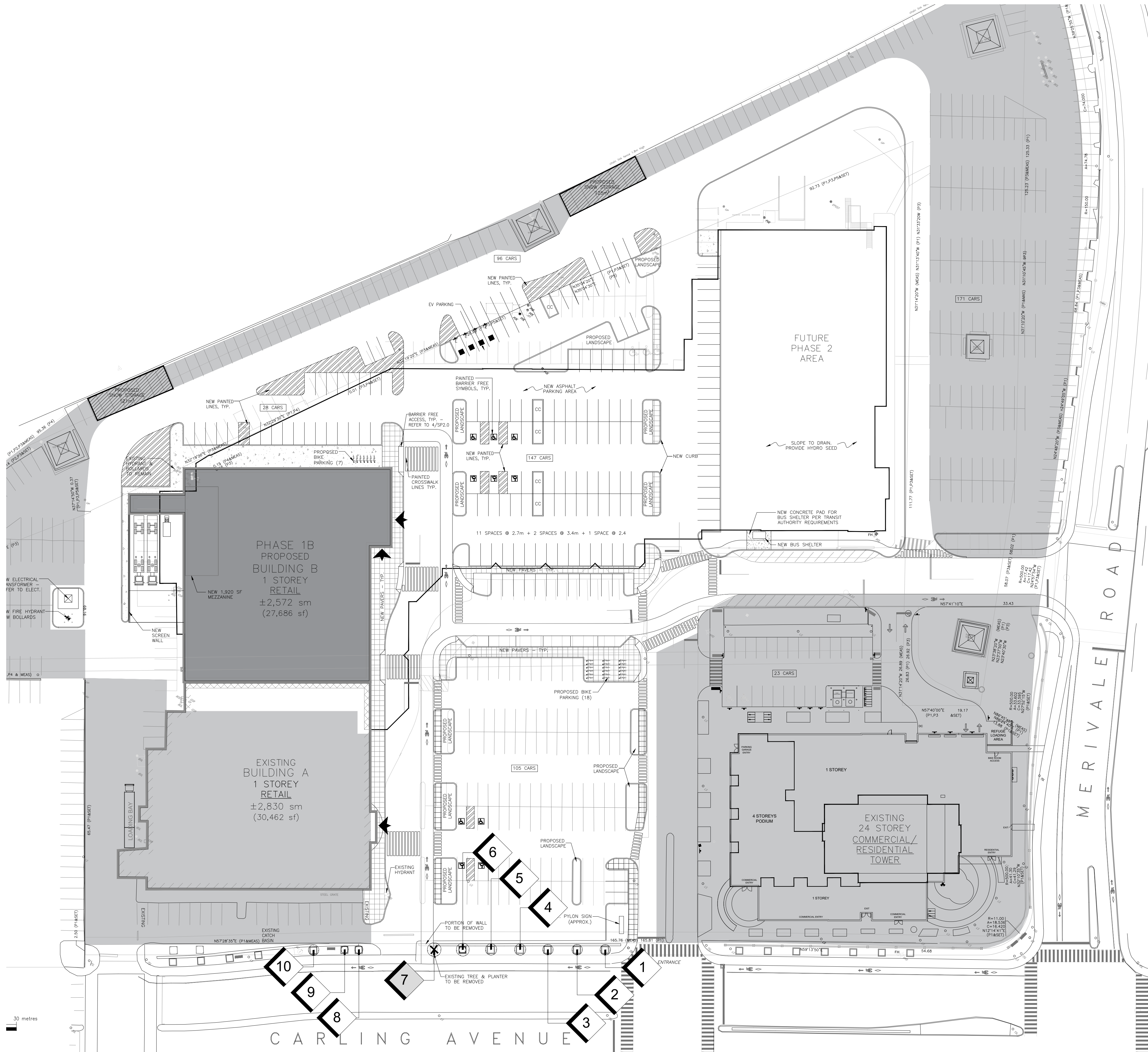
1 TREE INVENTORY, PROTECTION, AND REMOVALS PLAN SCALE: 1:500
