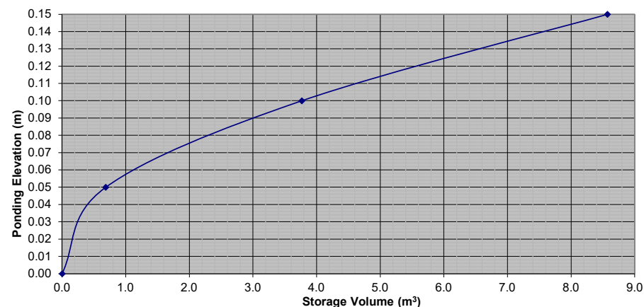
Stage Storage Curve: Area A-1.1 Controlled Roof Drain RD-7
