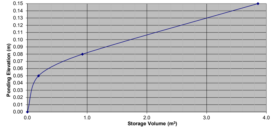
Stage Storage Curve: Area A-1.1 Controlled Roof Drain RD-13
