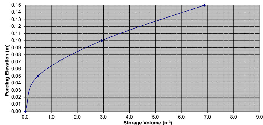
Stage Storage Curve: Area A-1.1 Controlled Roof Drain RD-10
