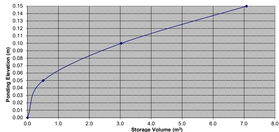
Stage Storage Curve: Area A-1.1 Controlled Roof Drain RD-9
