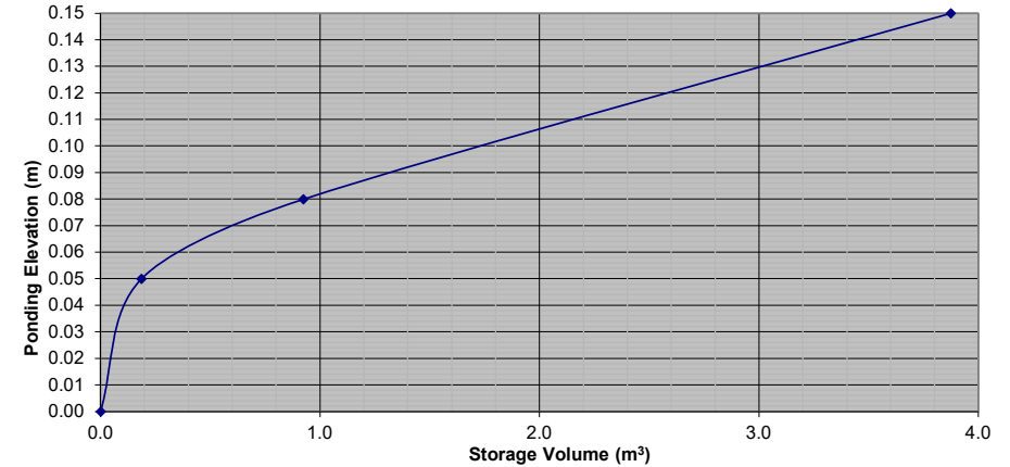
Stage Storage Curve: Area A-1.1 Controlled Roof Drain RD-15
