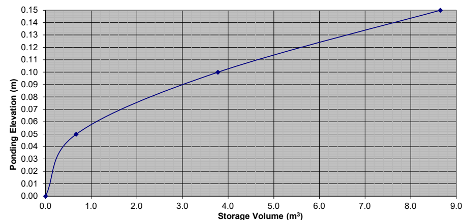
Stage Storage Curve: Area A-1.1 Controlled Roof Drain RD-3
