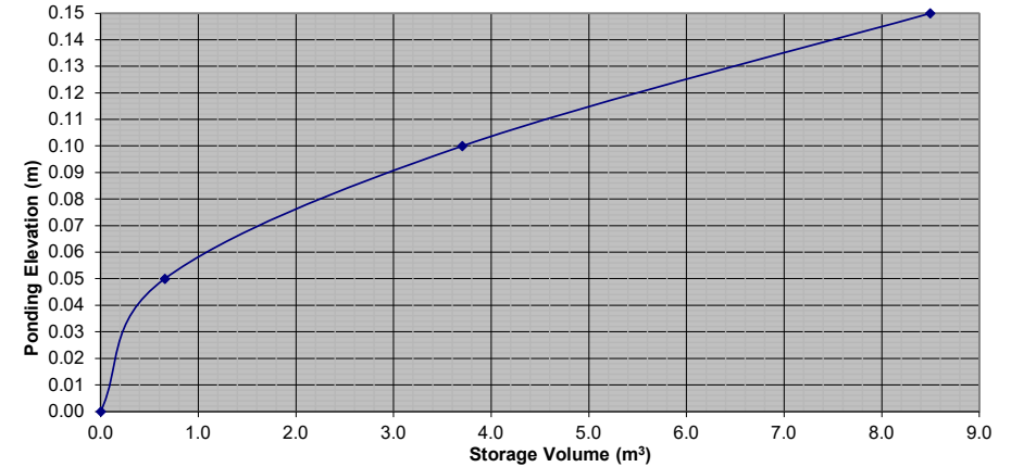
Stage Storage Curve: Area A-1.1 Controlled Roof Drain RD-6
