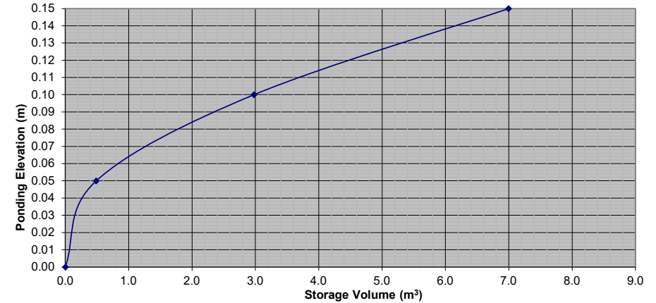
Stage Storage Curve: Area A-1.1 Controlled Roof Drain RD-1
