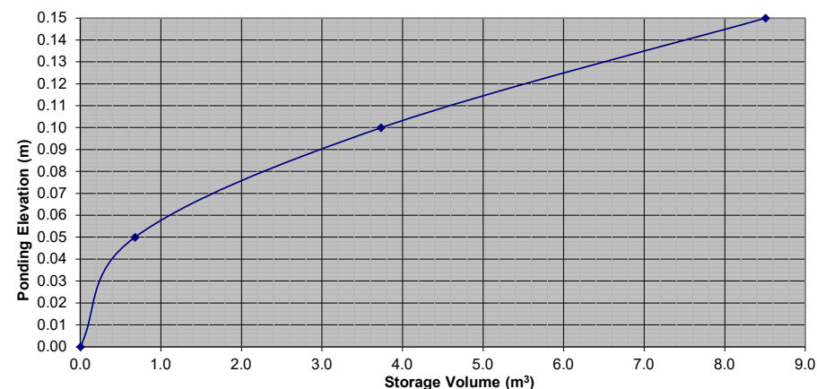
Stage Storage Curve: Area A-1.1 Controlled Roof Drain RD-8
