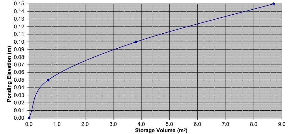
Stage Storage Curve: Area A-1.1 Controlled Roof Drain RD-5
