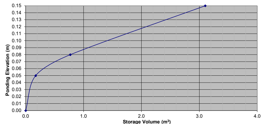
Stage Storage Curve: Area A-1.1 Controlled Roof Drain RD-12
