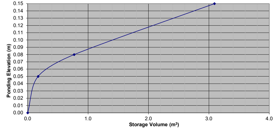
Stage Storage Curve: Area A-1.1 Controlled Roof Drain RD-11
