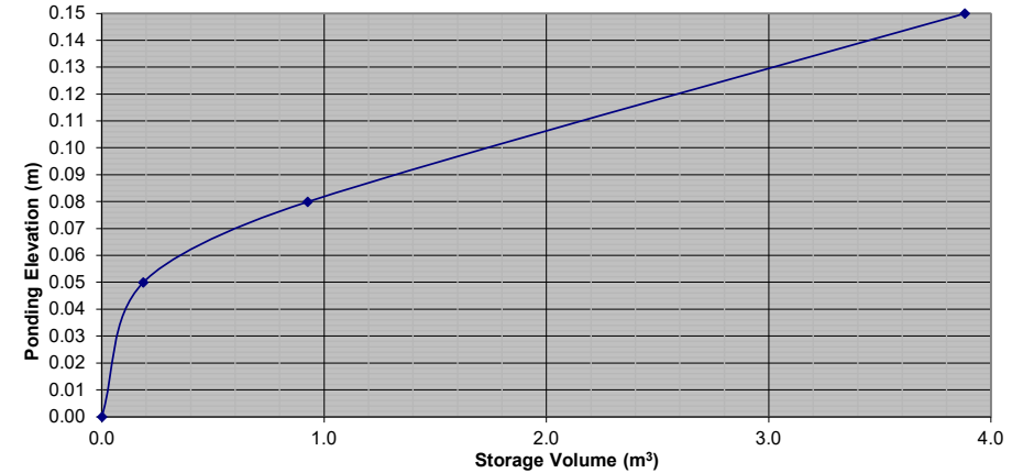
Stage Storage Curve: Area A-1.1 Controlled Roof Drain RD-14
