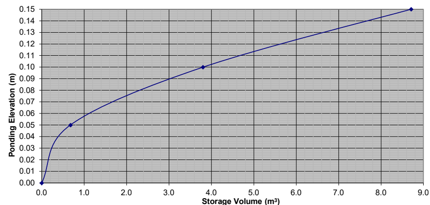
Stage Storage Curve: Area A-1.1 Controlled Roof Drain RD-4
