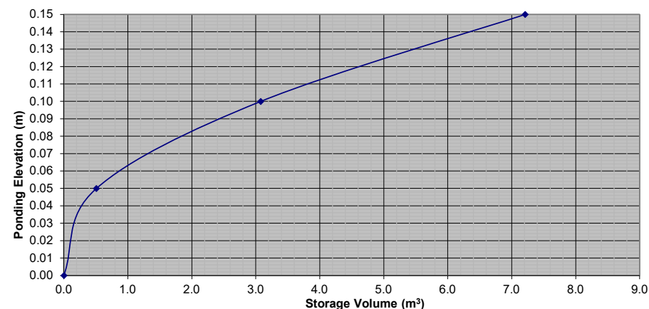
Stage Storage Curve: Area A-1.1 Controlled Roof Drain RD-2
