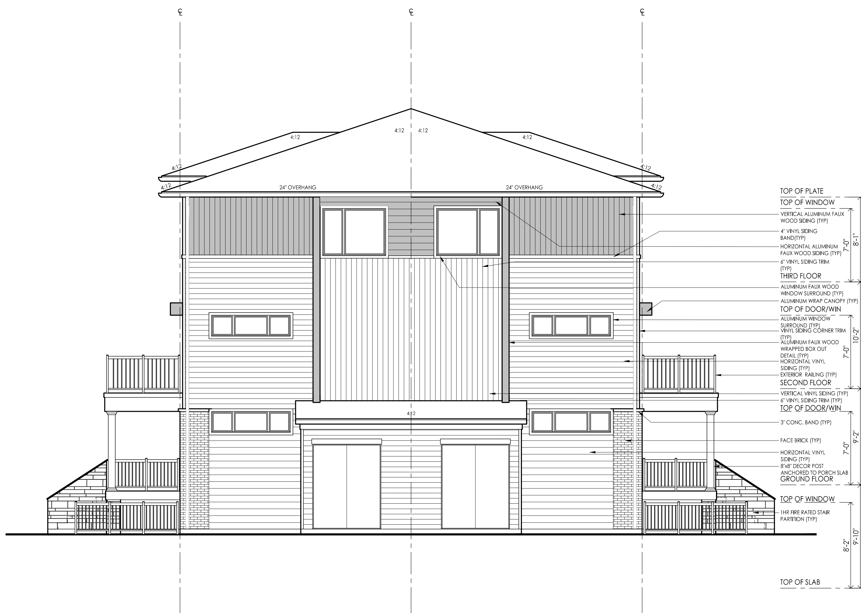
SIDE ELEVATION - METRO TOWN TYPICAL BLOCK
