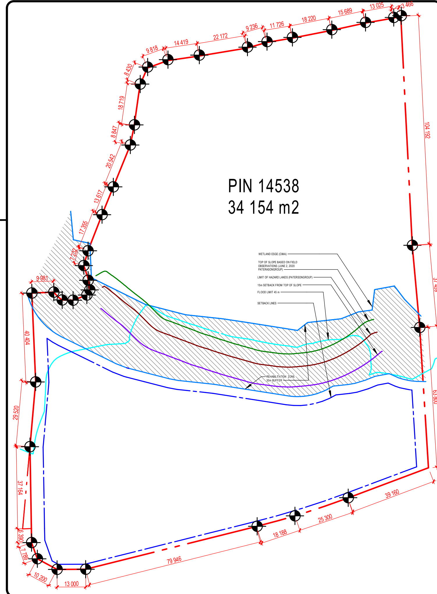
KEY PLAN - PROPERTY BOUNDARY 1:1000
