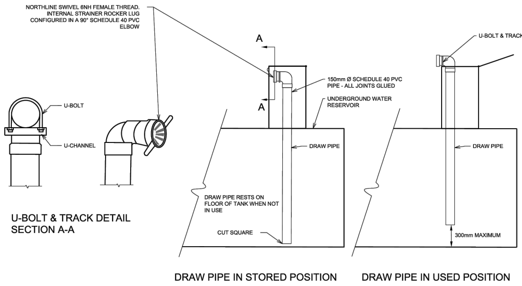
DRAW PIPE IN STORED POSITION DRAW PIPE IN USED POSITION
