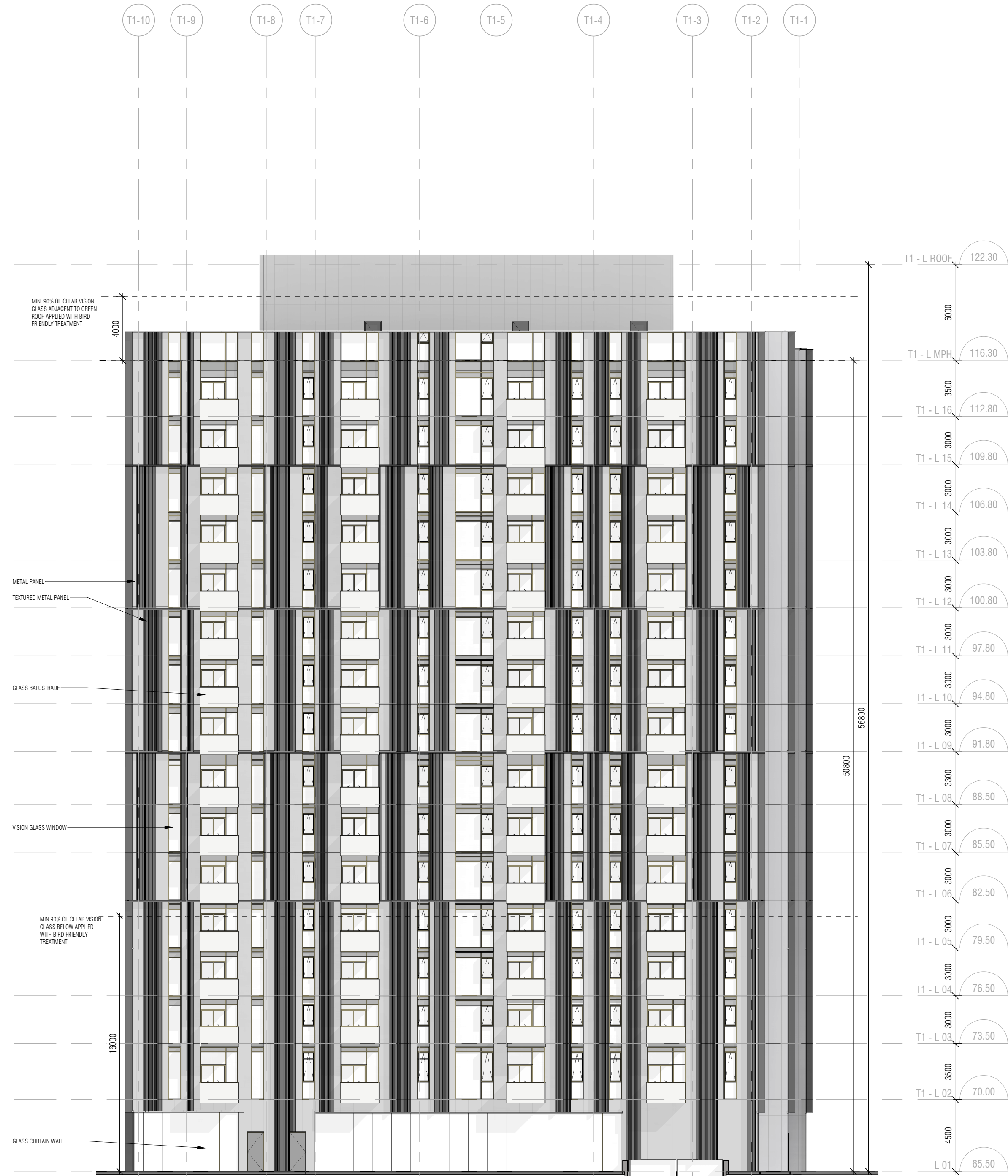
4 WEST TOWER WEST ELEVATION A302-T1 1:200
