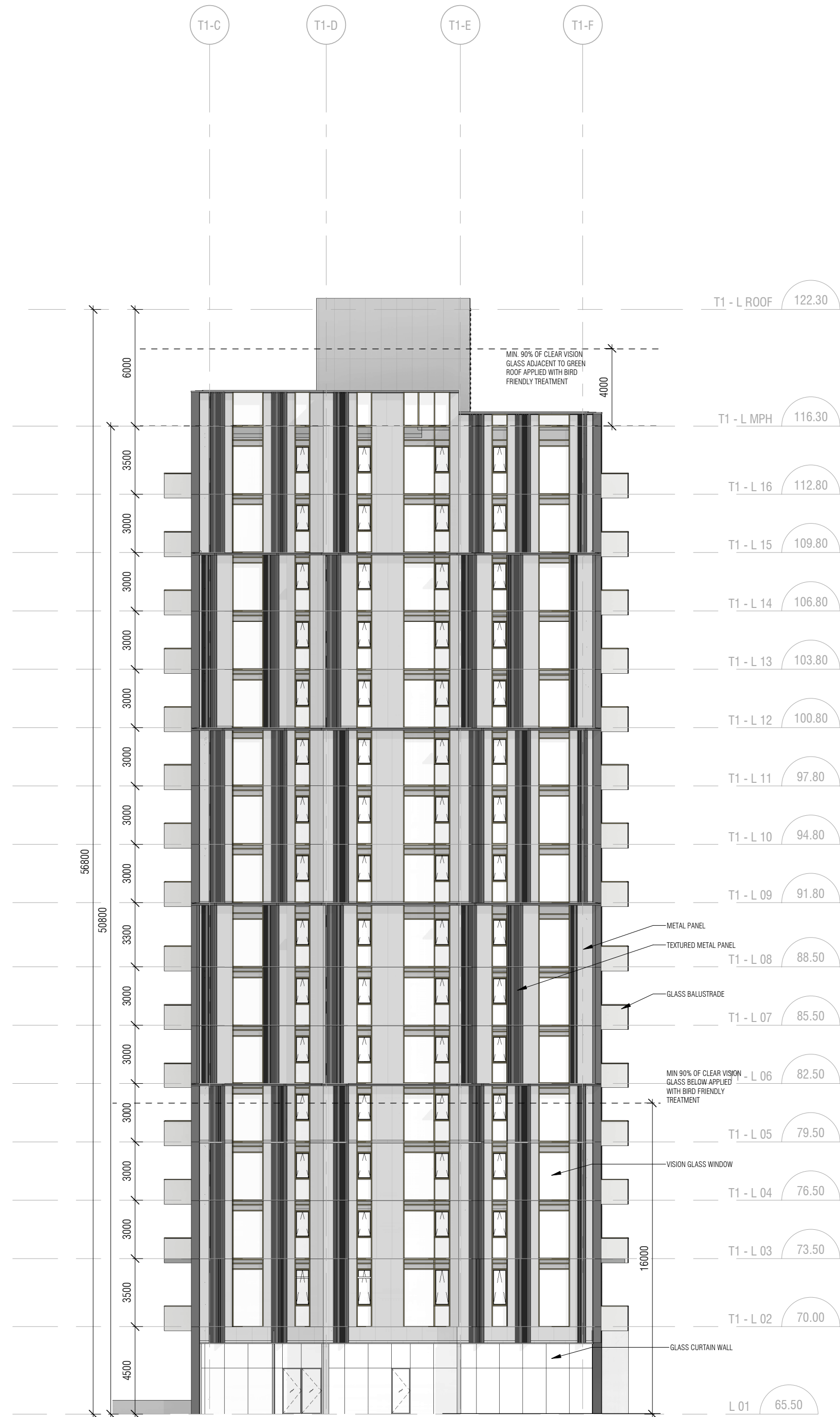
2 WEST TOWER SOUTH ELEVATION A302-T1 1:200
