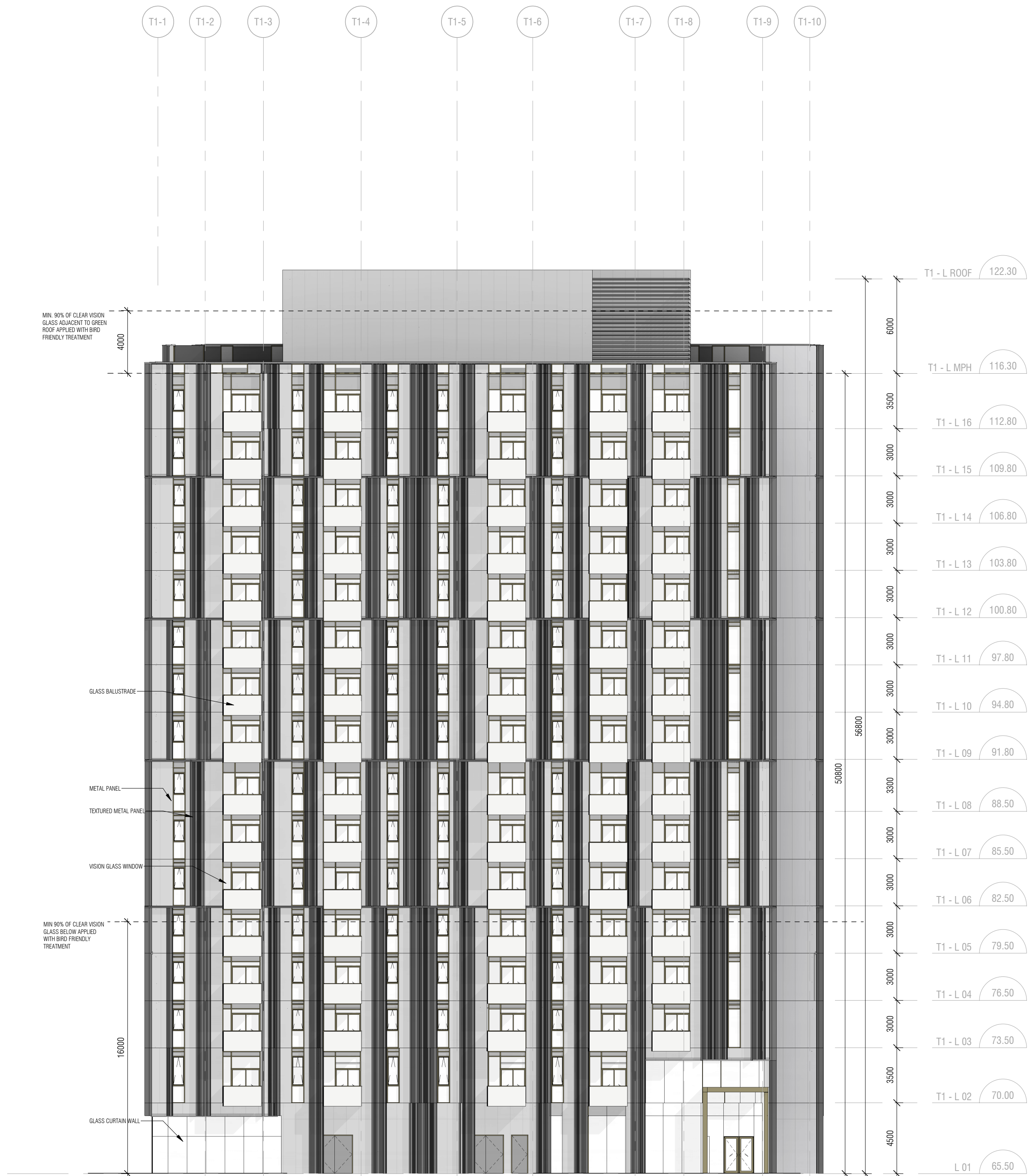
1 WEST TOWER EAST ELEVATION A302-T1 1:200
