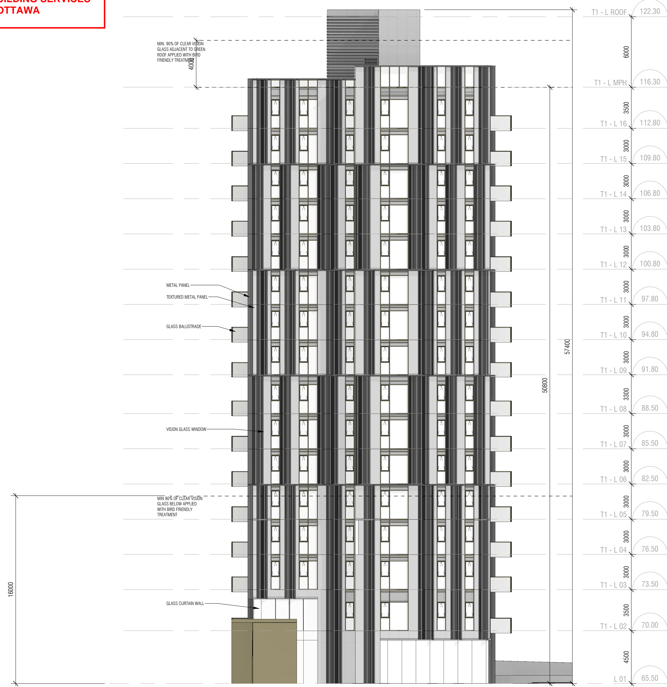
3 WEST TOWER NORTH ELEVATION A302-T1 1:200
