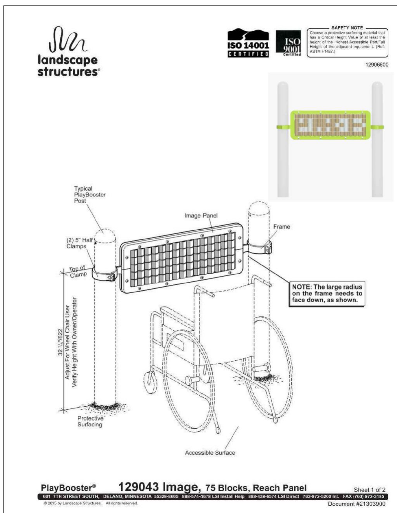
D3 L1100 TYPICAL PLAY PANEL AT AUTISM THERAPY TERRACE IMAGE
