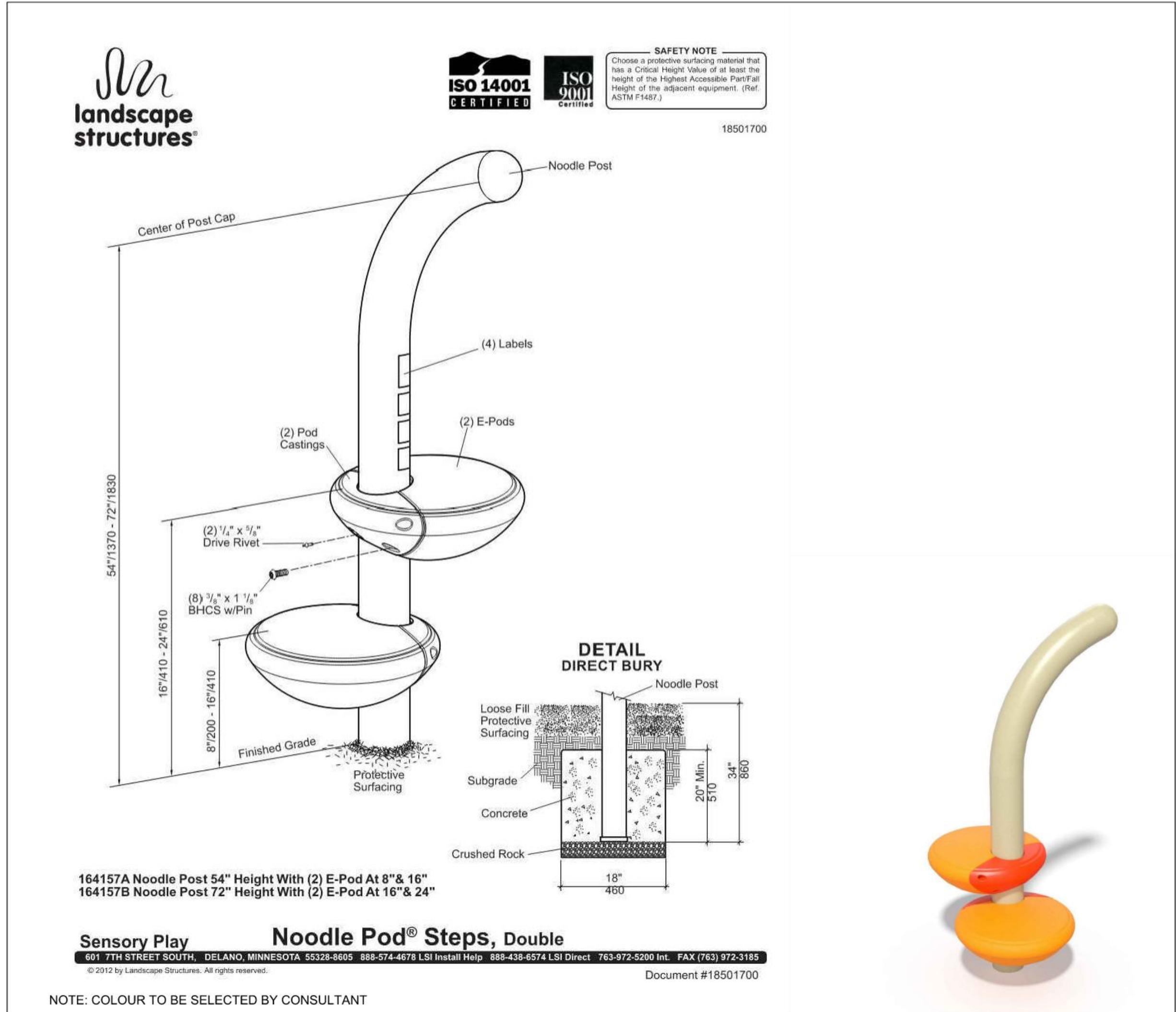
D2 L1100 TYPICAL POD STATION AT AUTISM THERAPY TERRACE MANUFACTURER'S RENDERING
