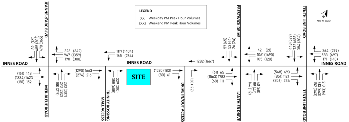
Figure 15: 2025 Total Traffic Volumes
