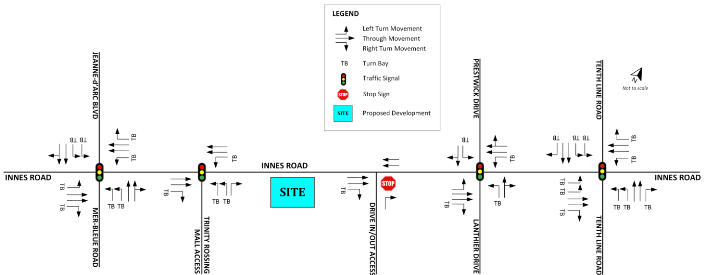
Figure 3: Existing Lane Configuration and Traffic Controls
