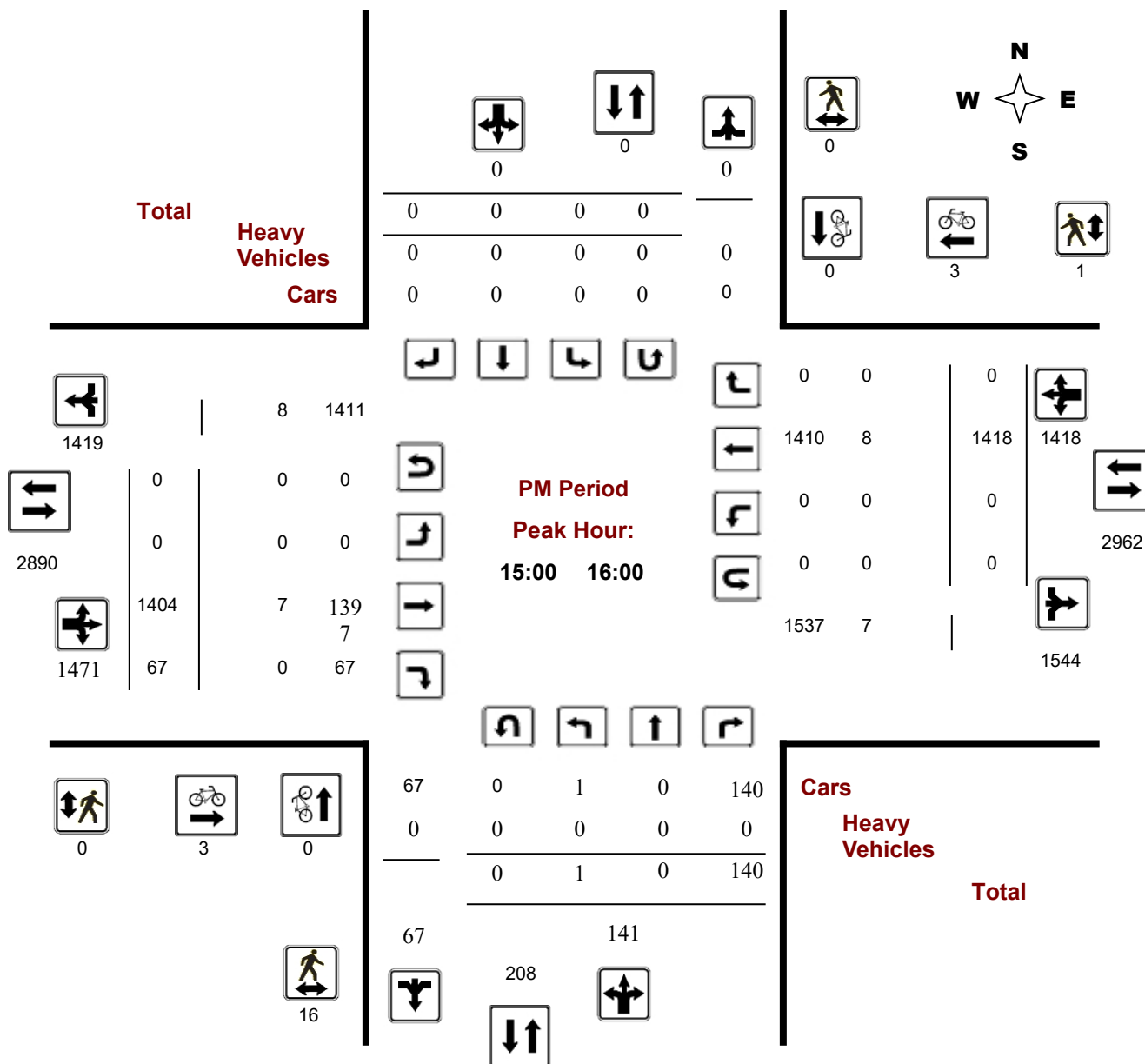
PM Period Peak Hour Diagram
