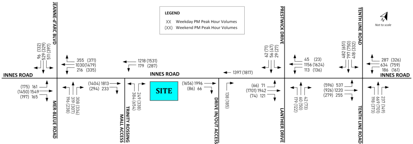
Figure 16: 2030 Total Traffic Volumes
