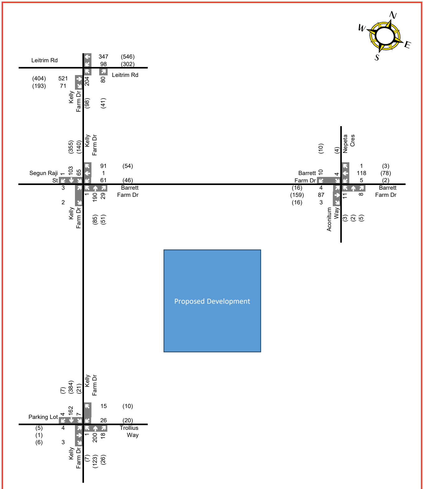
Figure 2-15 Existing (2024) Peak Hour Vehicular Volumes (Balanced)
