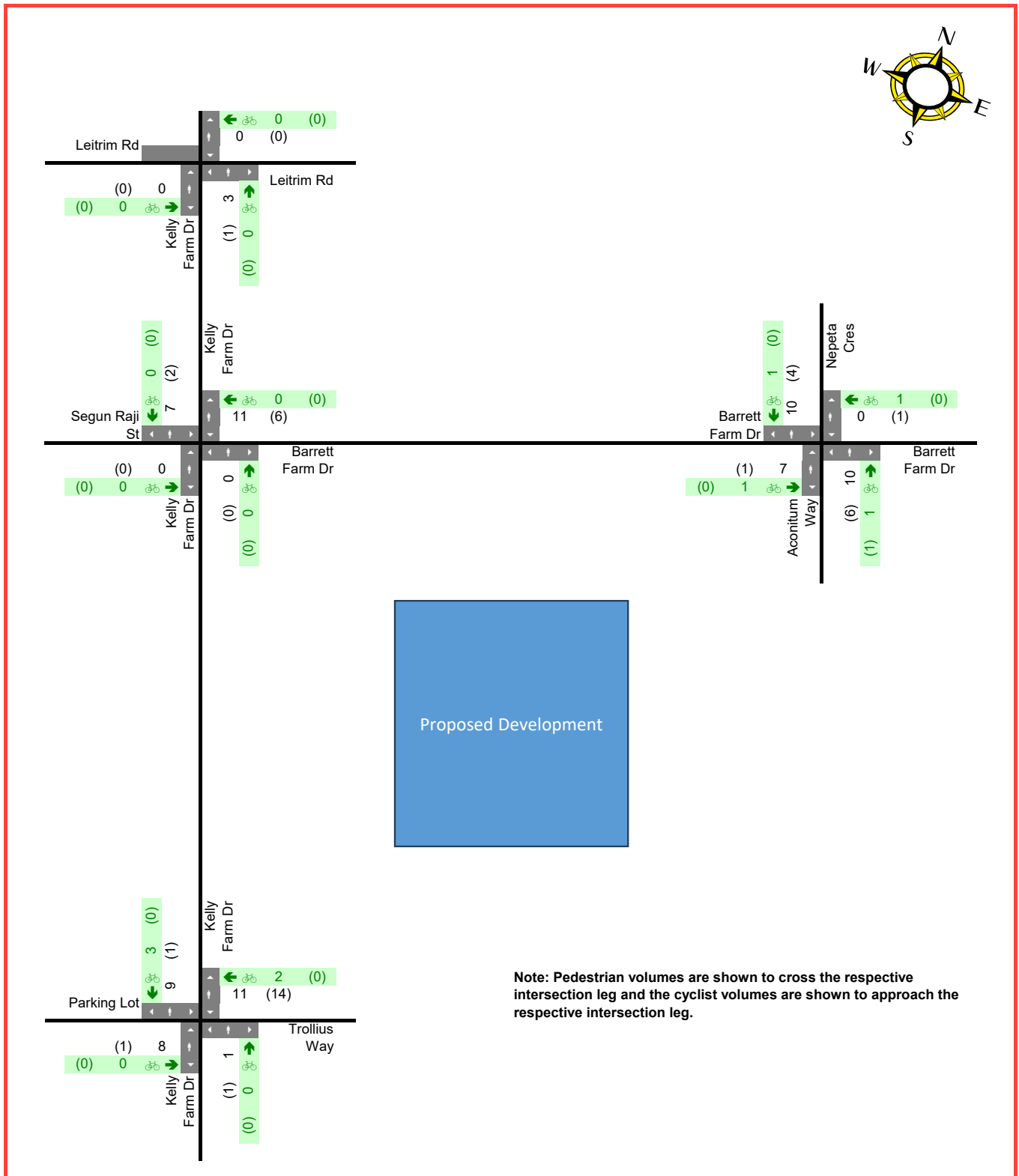
Figure 2-16 Existing (2024) Peak Hour Pedestrian and Cyclist Volumes
