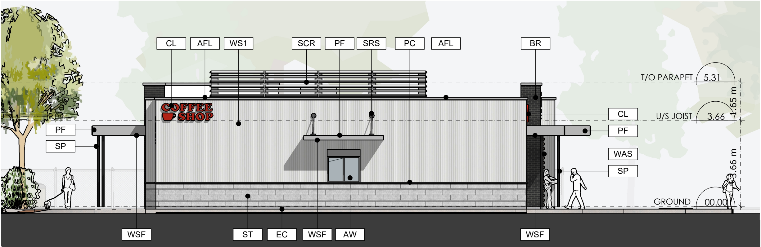
SOUTH ELEVATION
