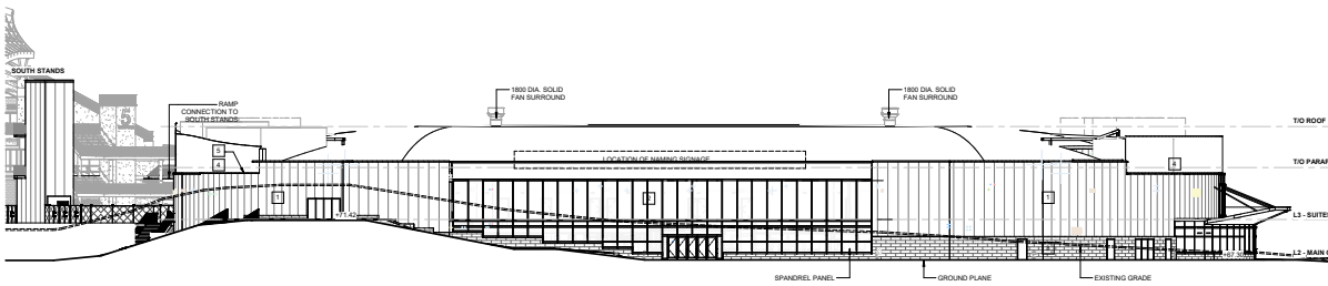
Proposed Event Centre east elevation (BBB, 2025).
