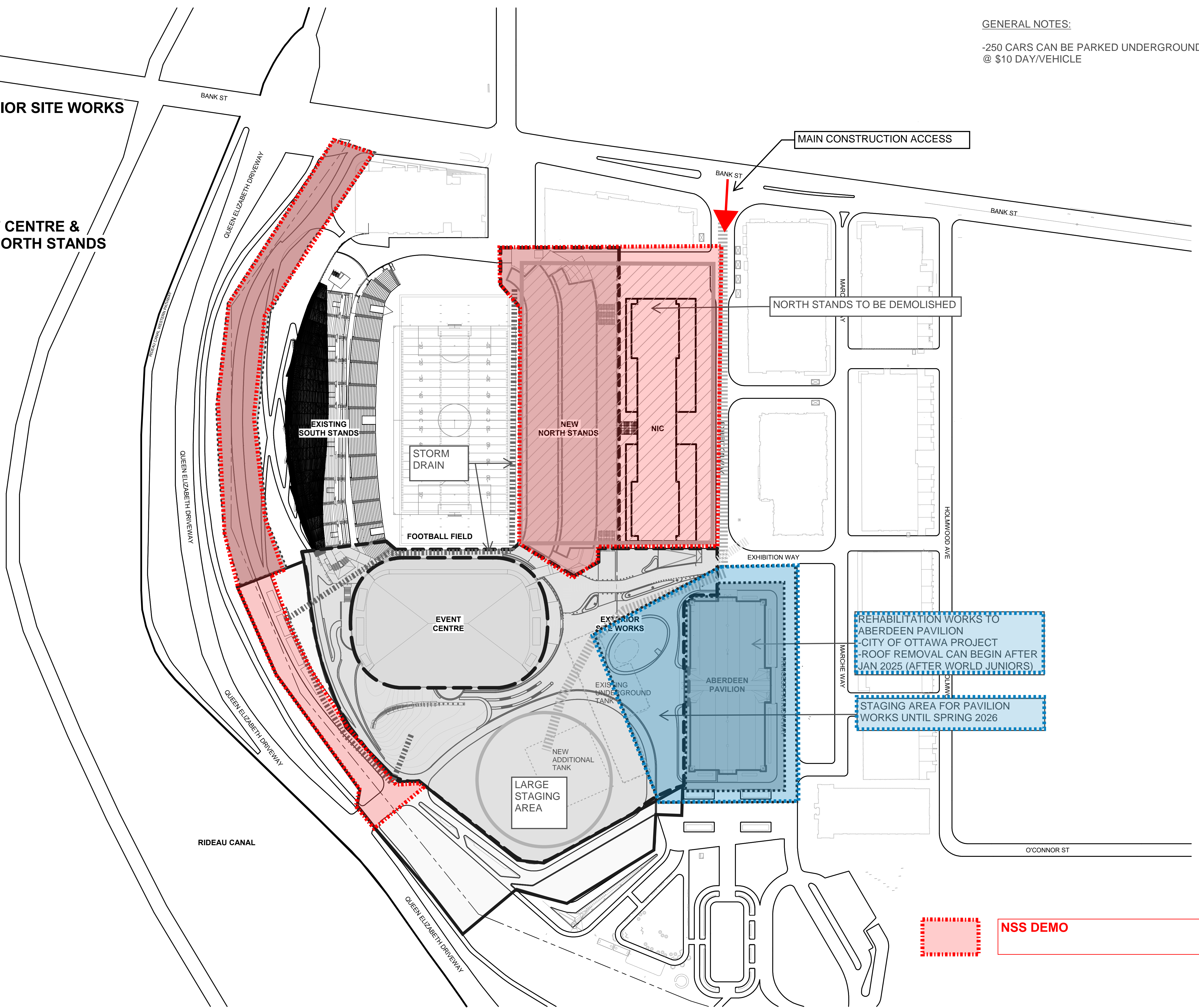
EXTENT OF EVENT CENTRE & NEW NORTH STANDS & EXTERIOR SITE WORKS 1:1000
