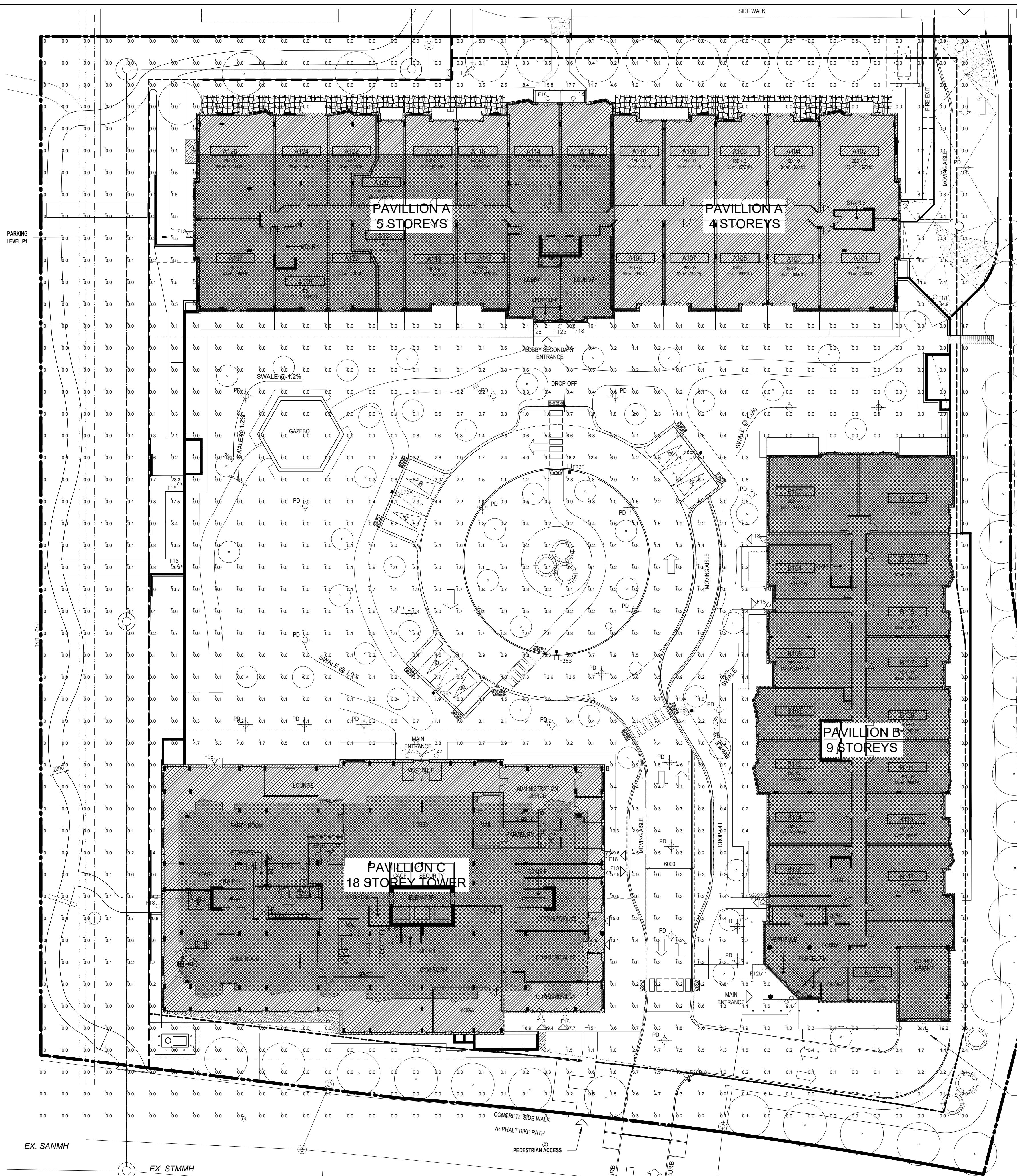
1 SITE PHOTOMETRICS PLAN EP-01 1:300
