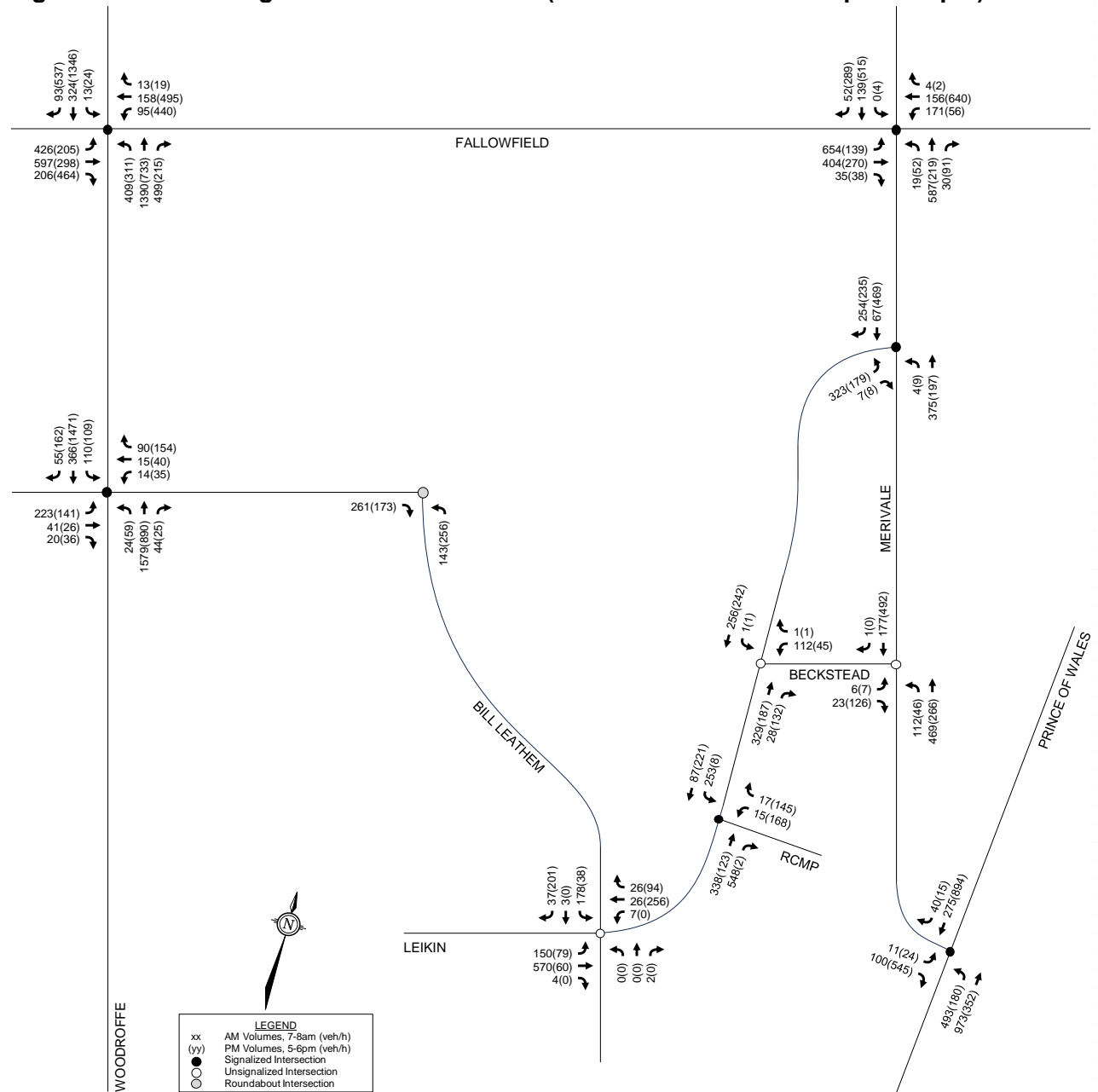
Figure 14: 2026 Background Traffic Volumes (7:00am-8:00am and 5:00pm-6:00pm)
