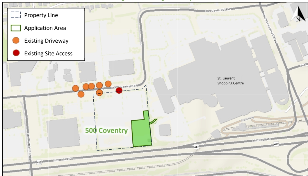
Figure 3: Existing Driveways
