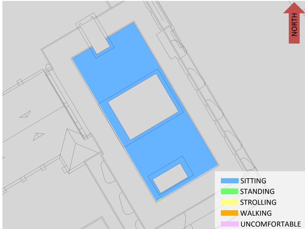
FIGURE 8: TYPICAL USE PERIOD – WIND COMFORT, ROOFTOP COMMON AMENITY TERRACE
