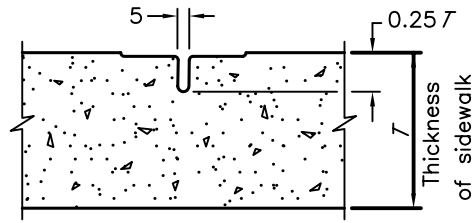
CONTRACTION JOINT
