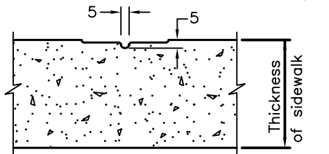
DUMMY JOINT
