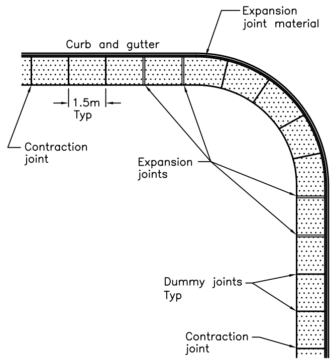
JOINT LAYOUT
