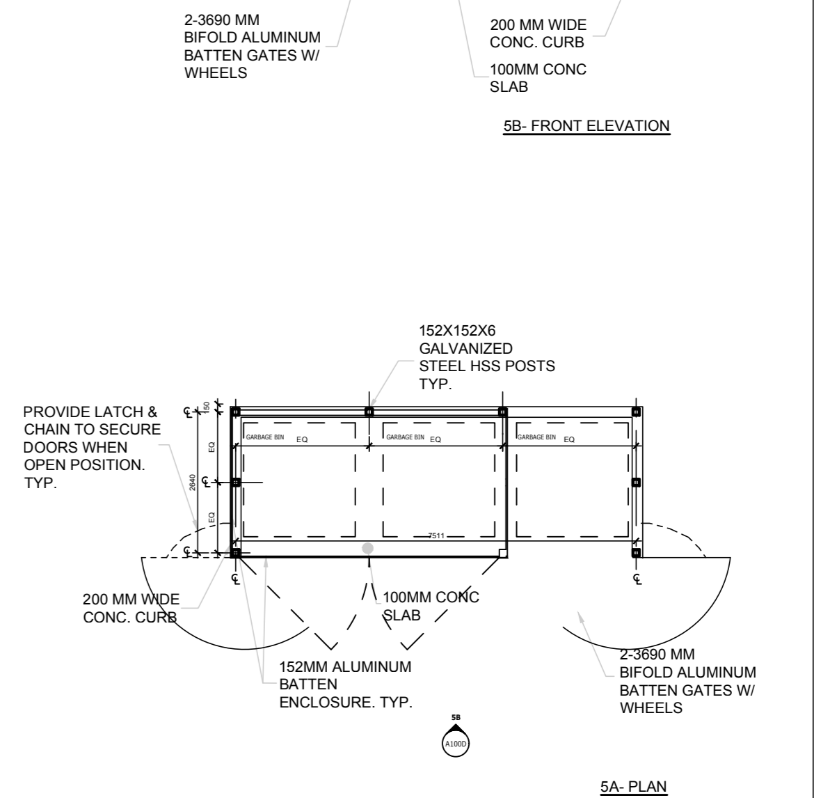
DETAIL - TYPICAL WASTE ENCLOSURE 1:500
