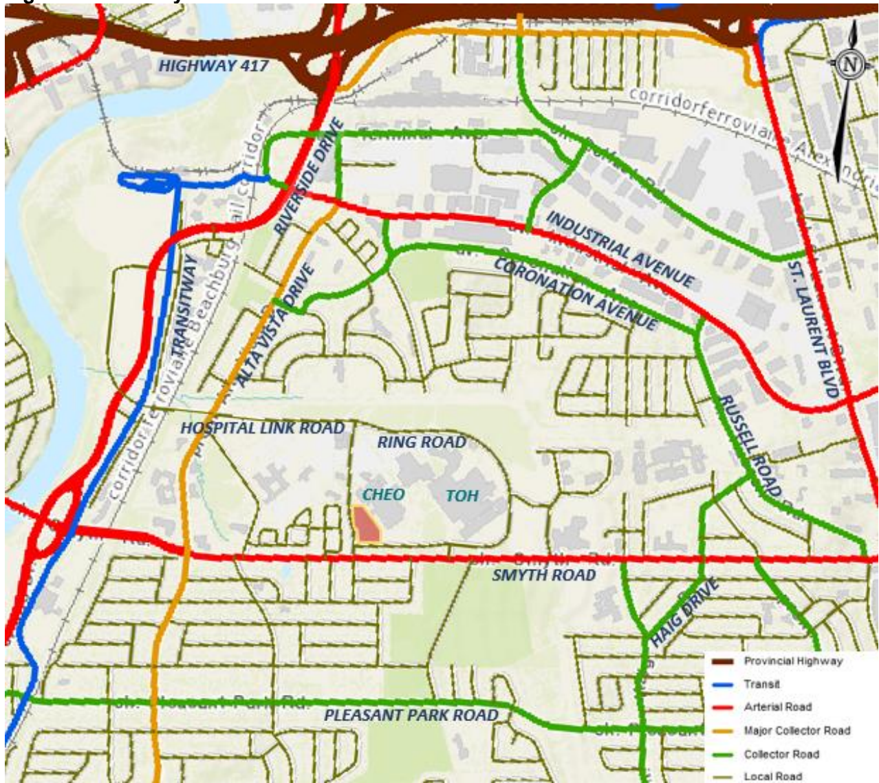
Figure 3: Roadway Network
