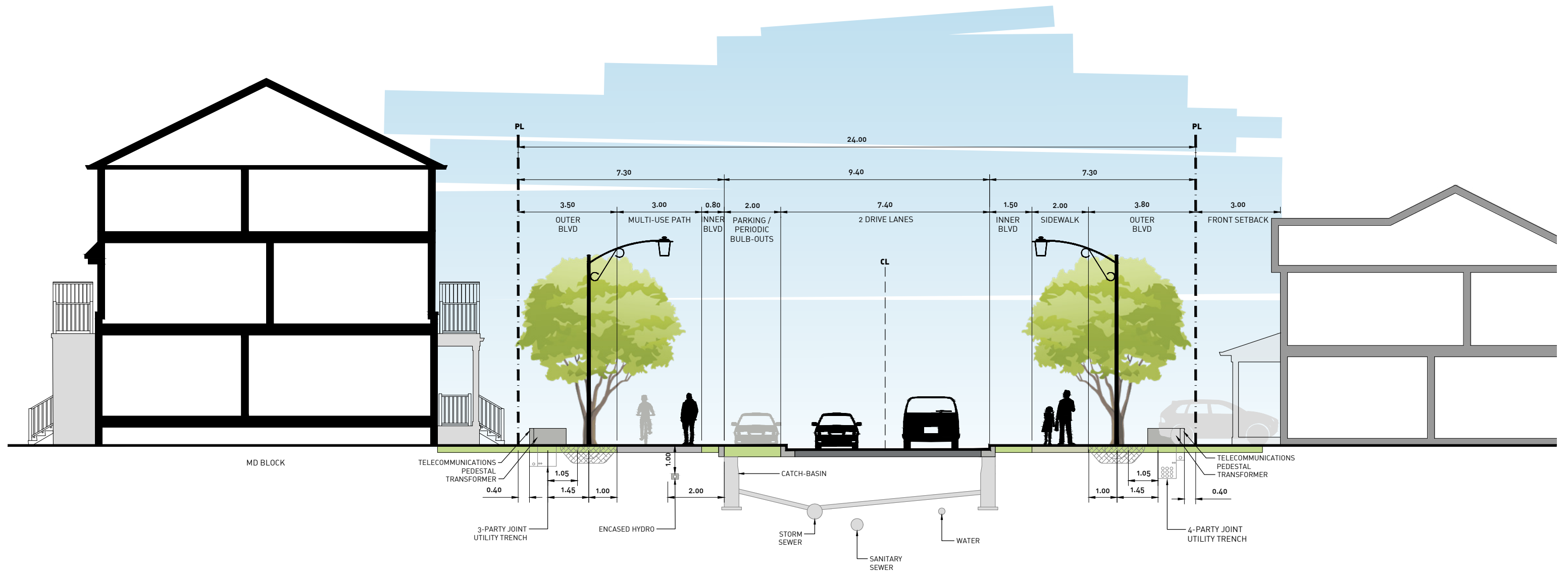
Figure 11 24.0m Collector Road (Conservancy Drive) Right-Of-Way Section
