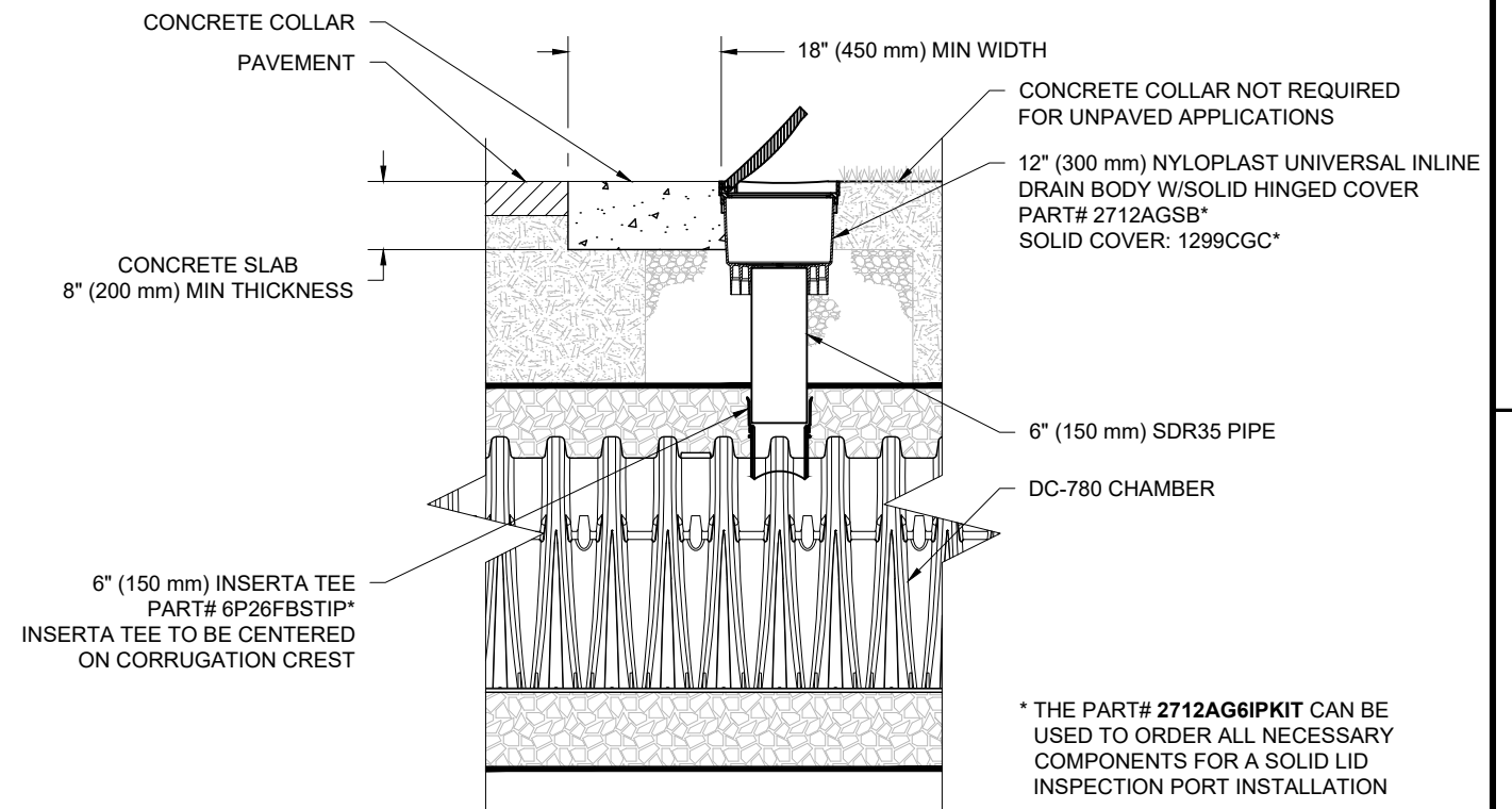
DC-780 6" (150 mm) INSPECTION PORT DETAIL NTS
