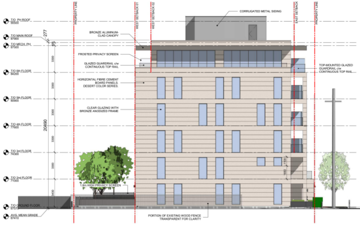
SOUTH ELEVATION
