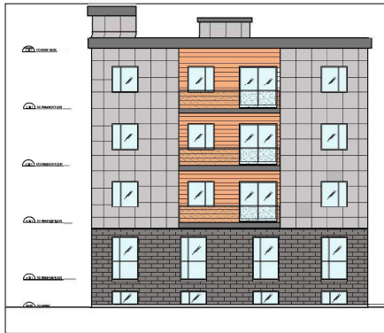
1 REAR (SOUTH) FACADE SCALE = 1/8" = 1'-0"
