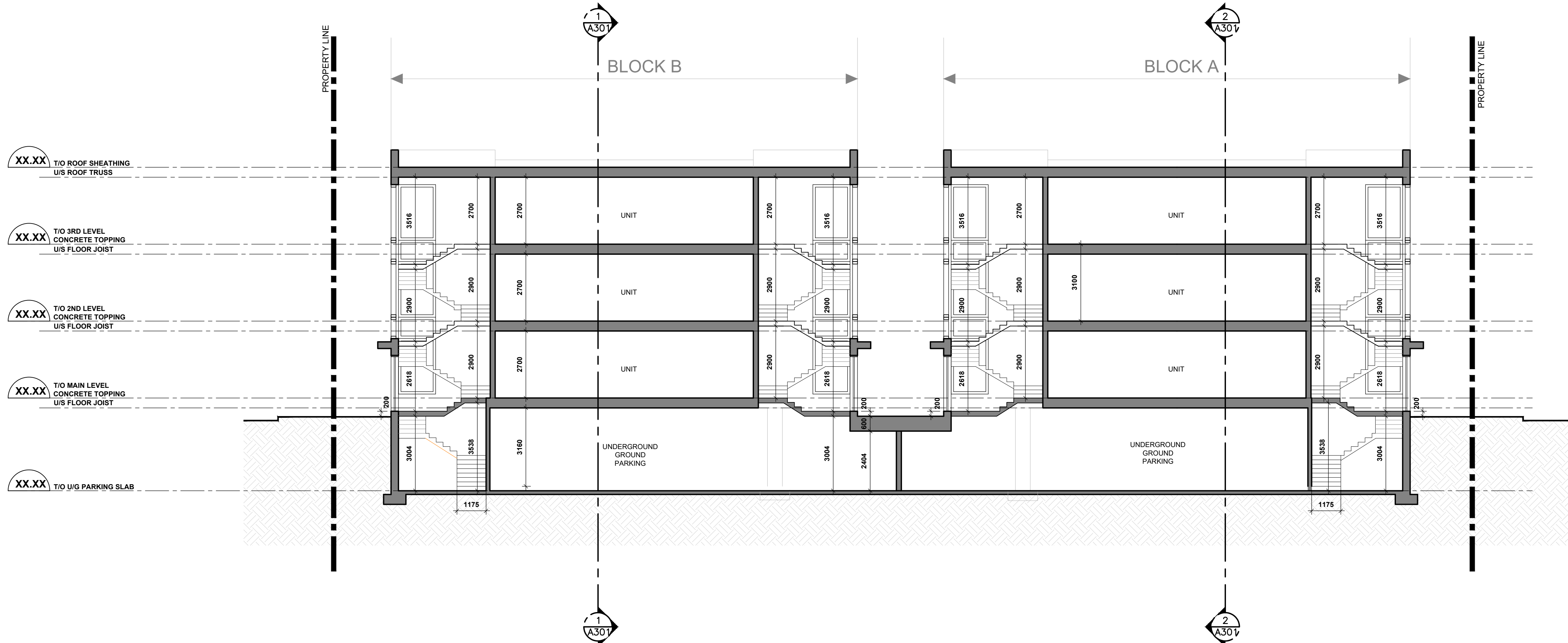
1 BUILDING SECTION (THROUGH OPEN STAIRS) SCALE = 1:100
