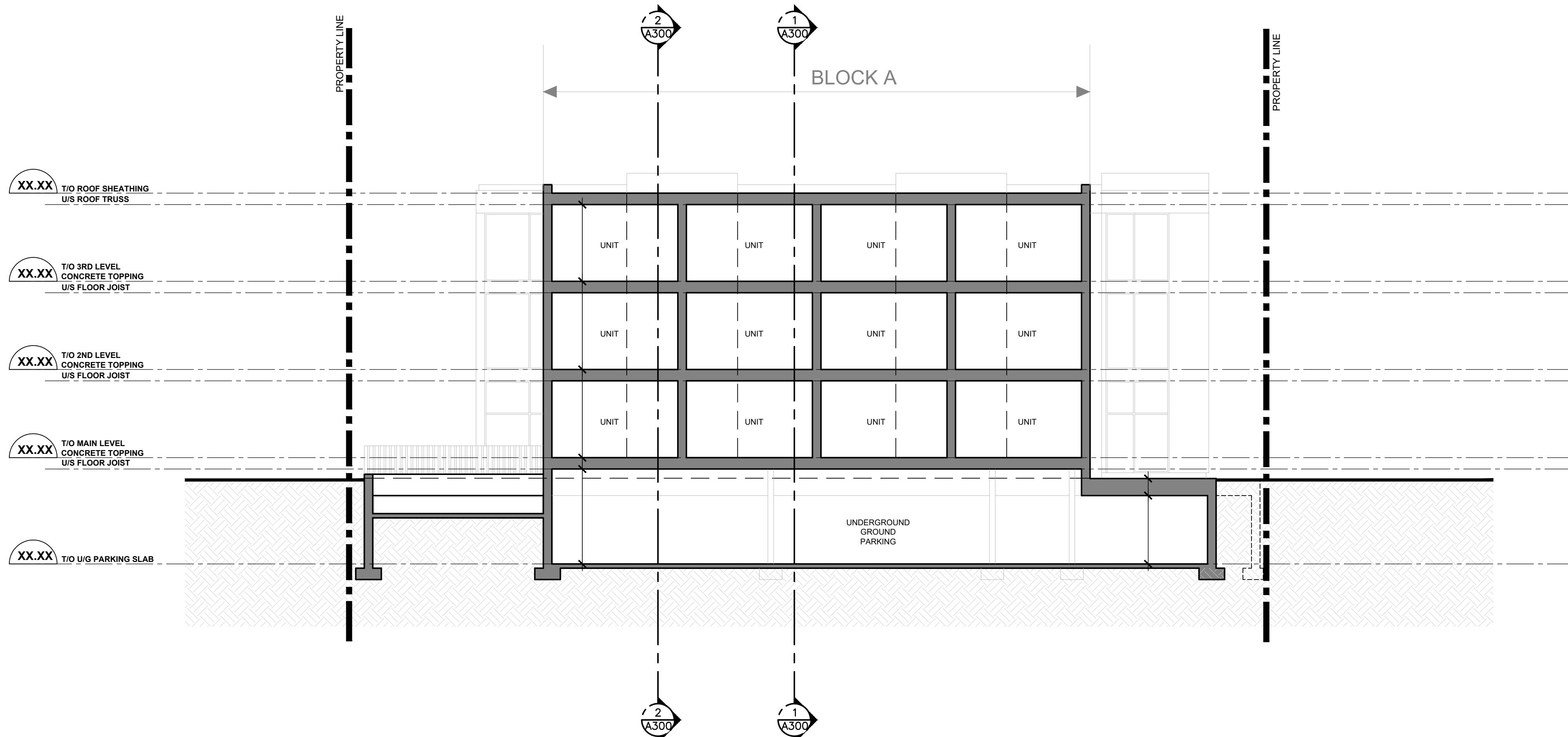
2 BUILDING_A SECTION (LOOKING WEST) SCALE = 1:100
