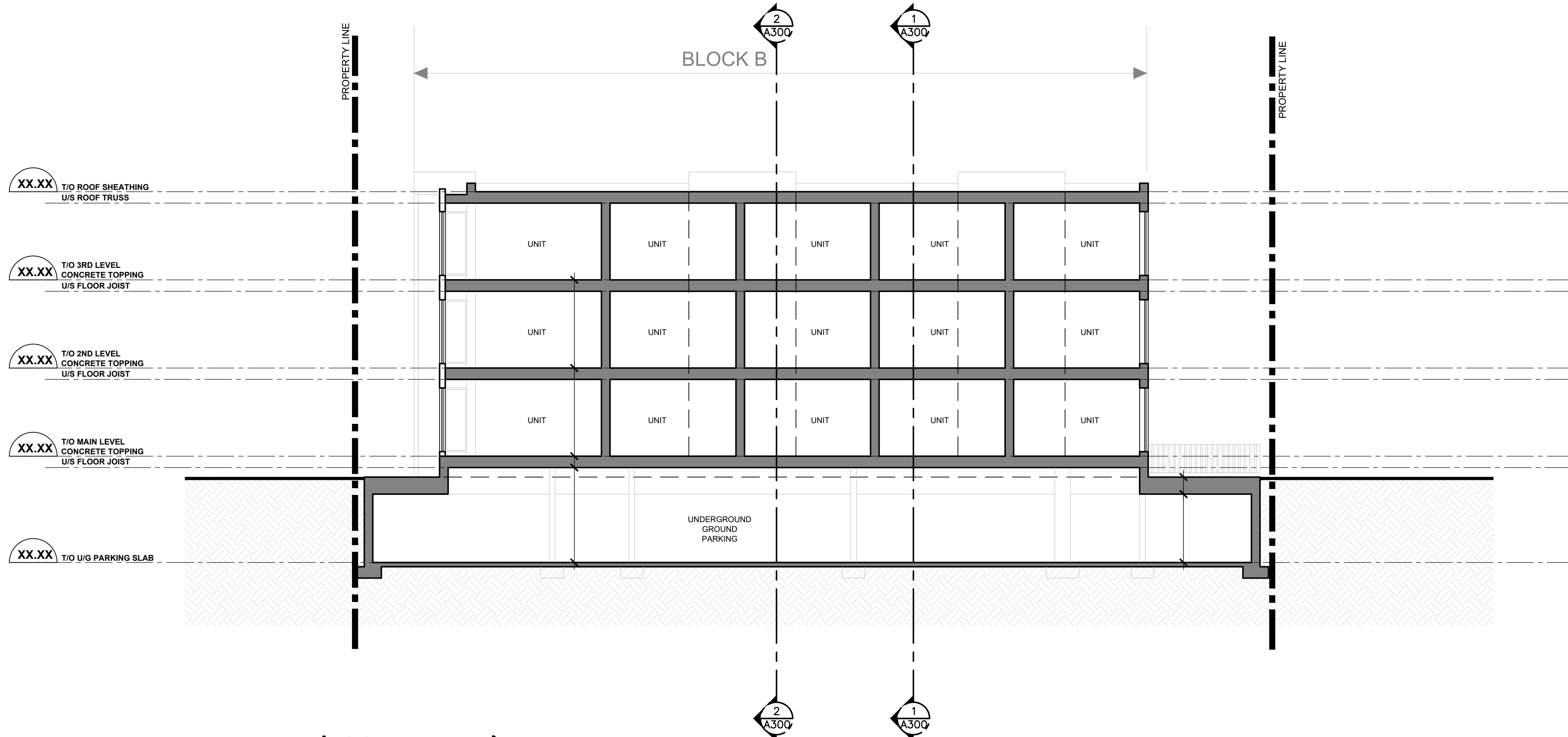
1 BUILDING_B SECTION (LOOKING EAST) SCALE = 1:100
