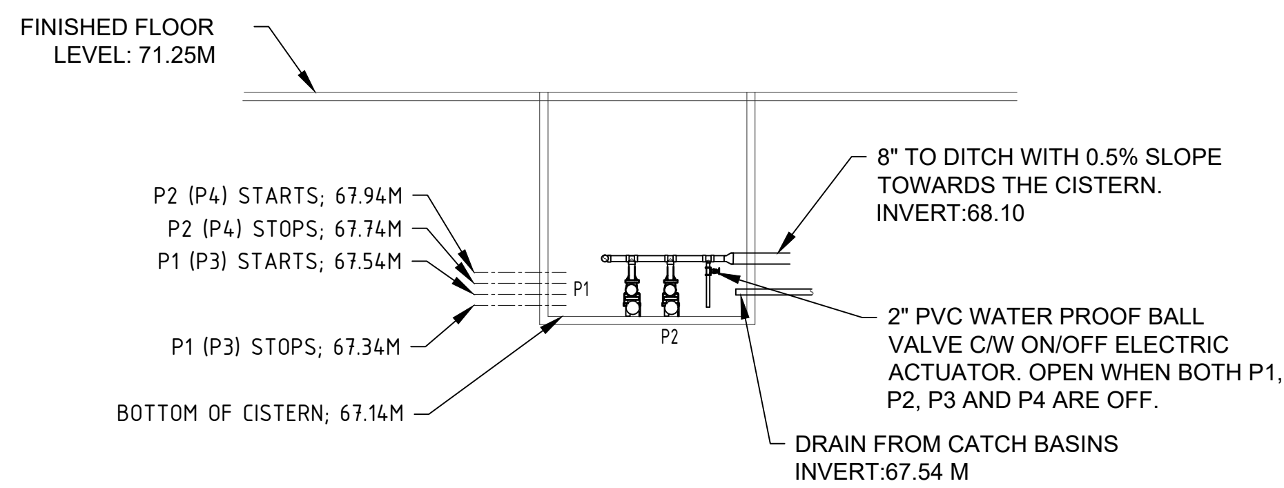
SECTION THROUGH B-B
