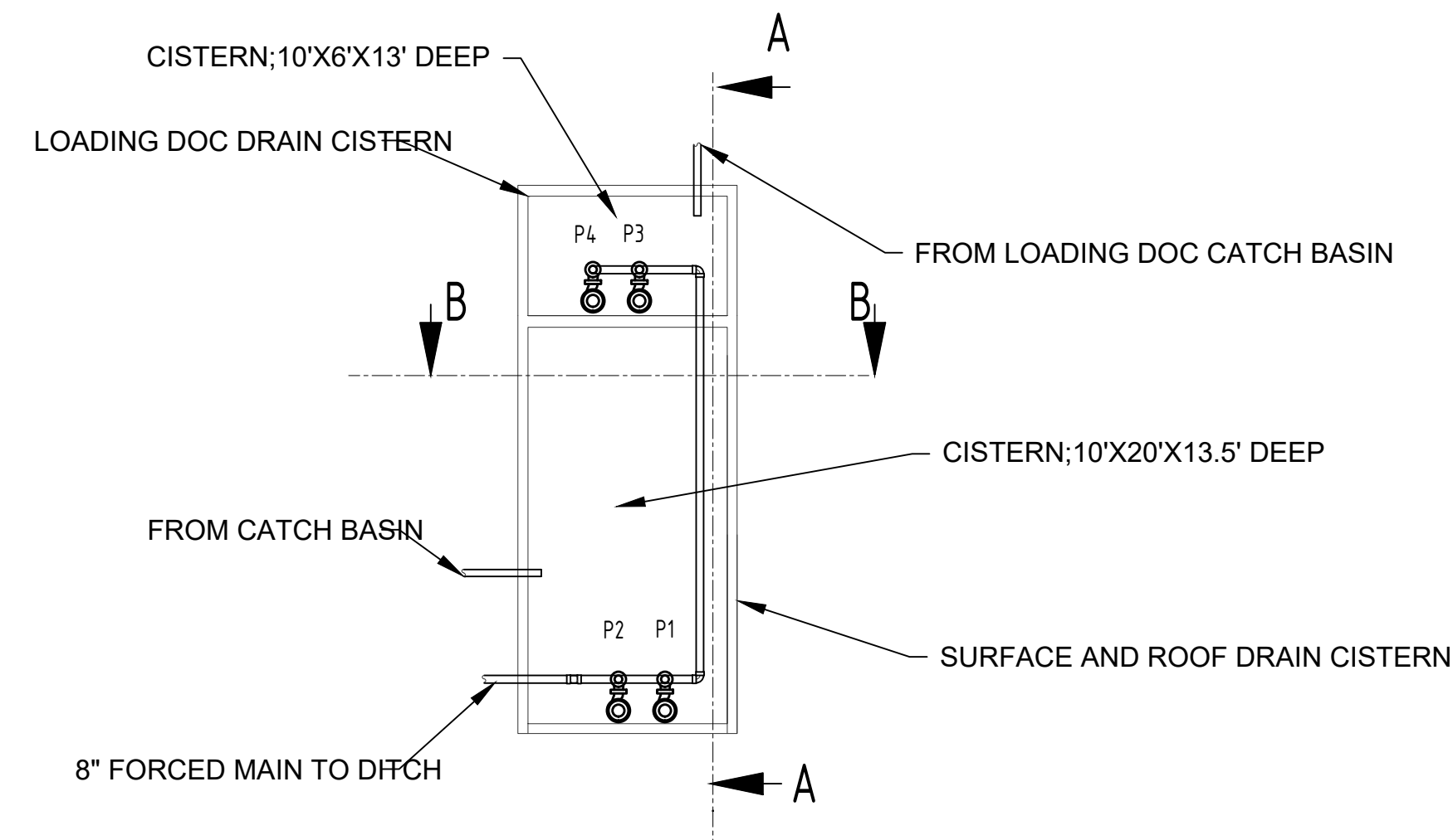
PLAN VIEW OF SURFACE & RAIN DRAIN CISTERN AND LOADING DOC DRAIN CISTERN
