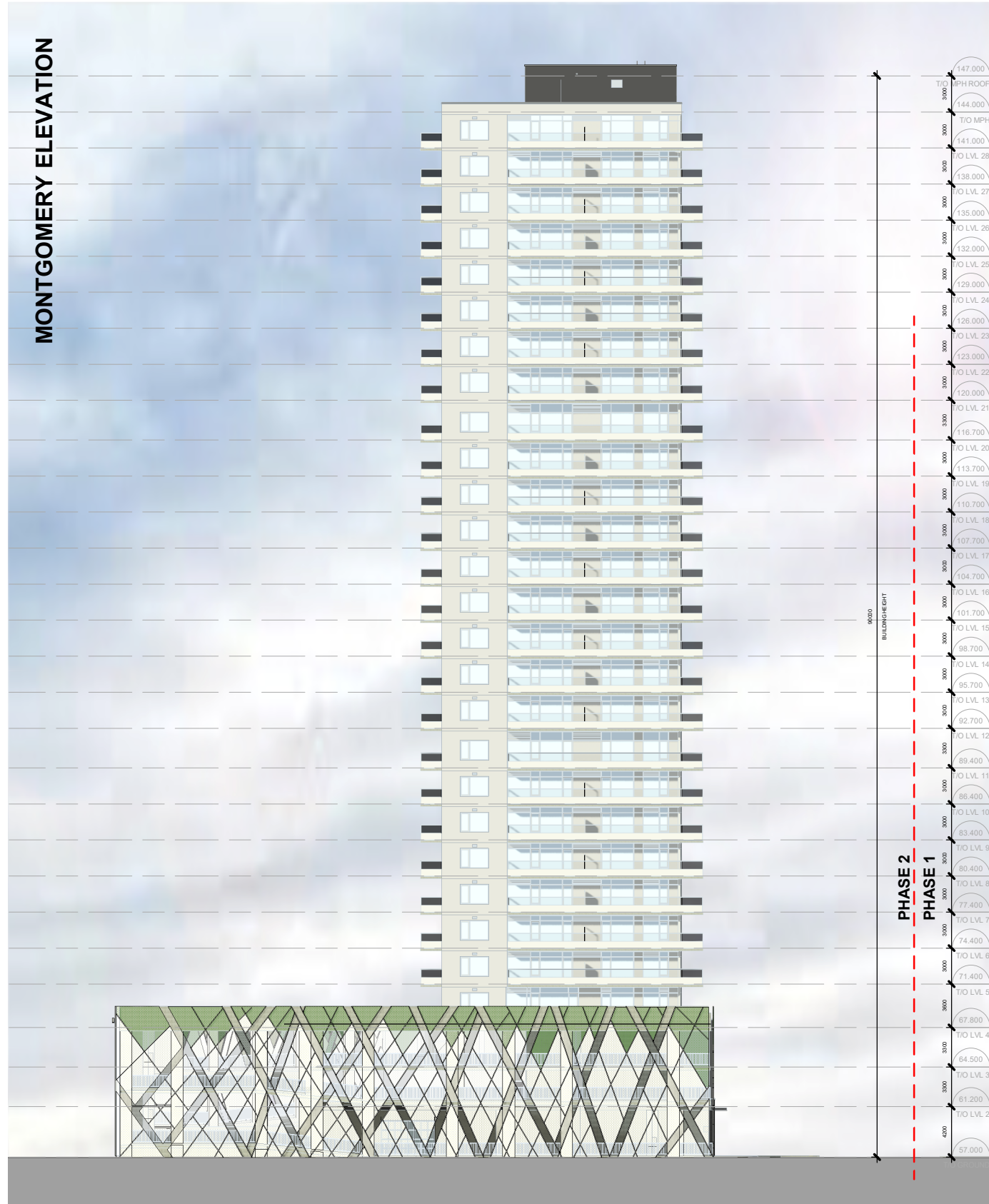
MONTGOMERY ELEVATION
