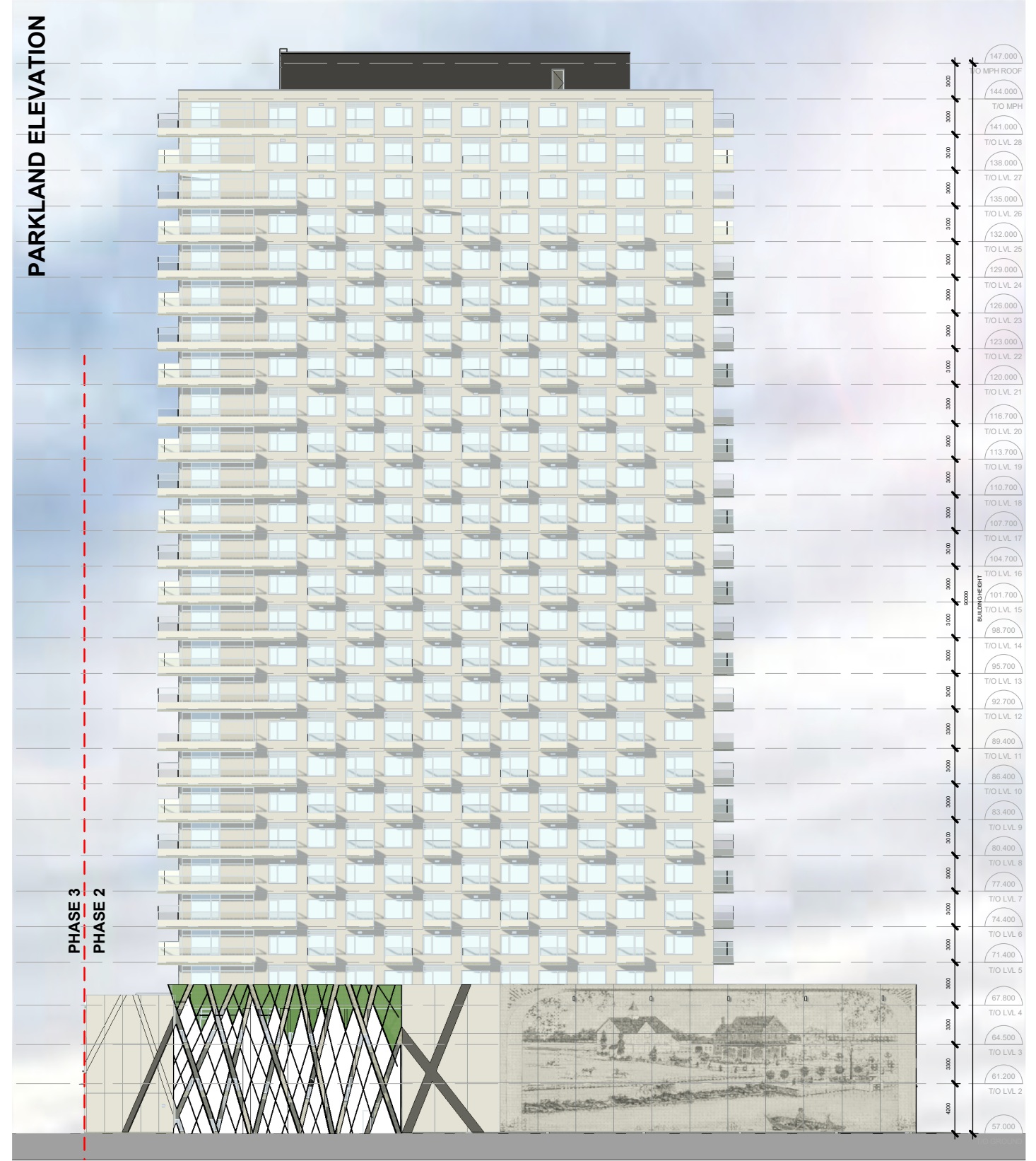
PARKLAND ELEVATION
