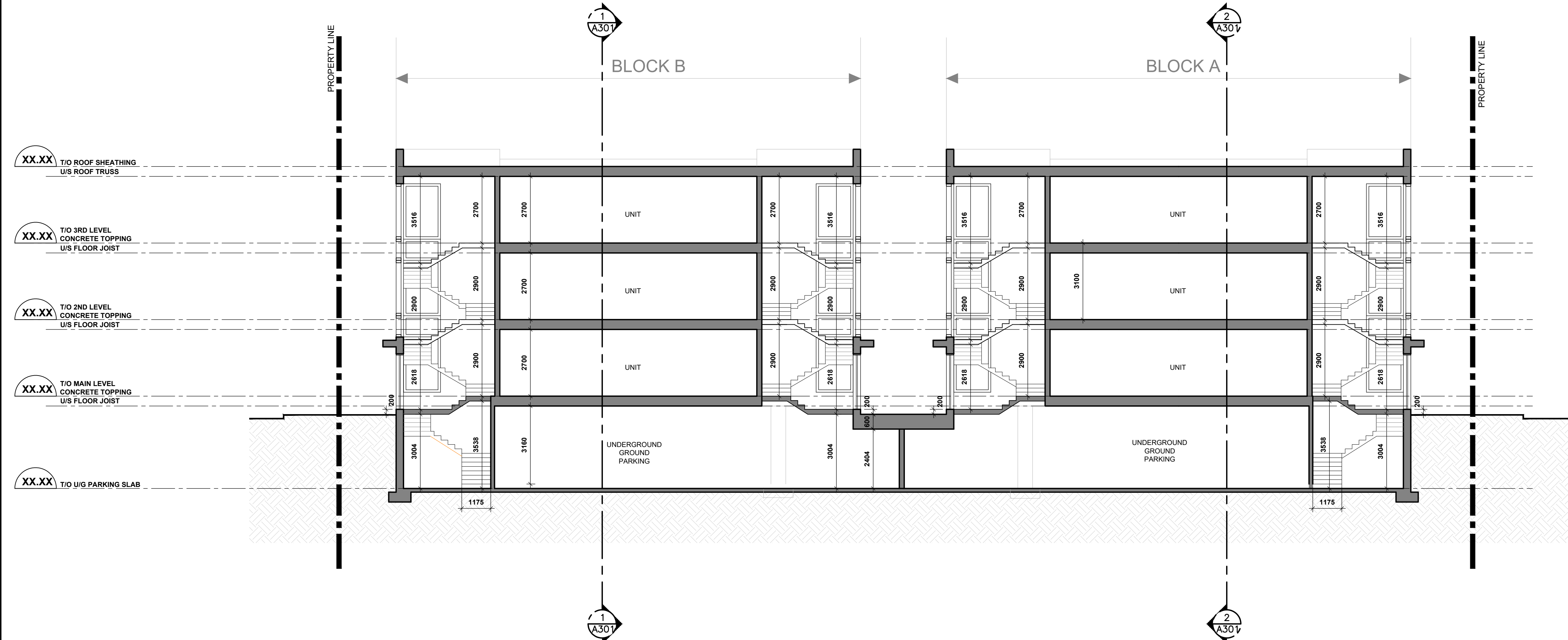
1 BUILDING SECTION (THROUGH OPEN STAIRS) A-300 SCALE = 1:100
