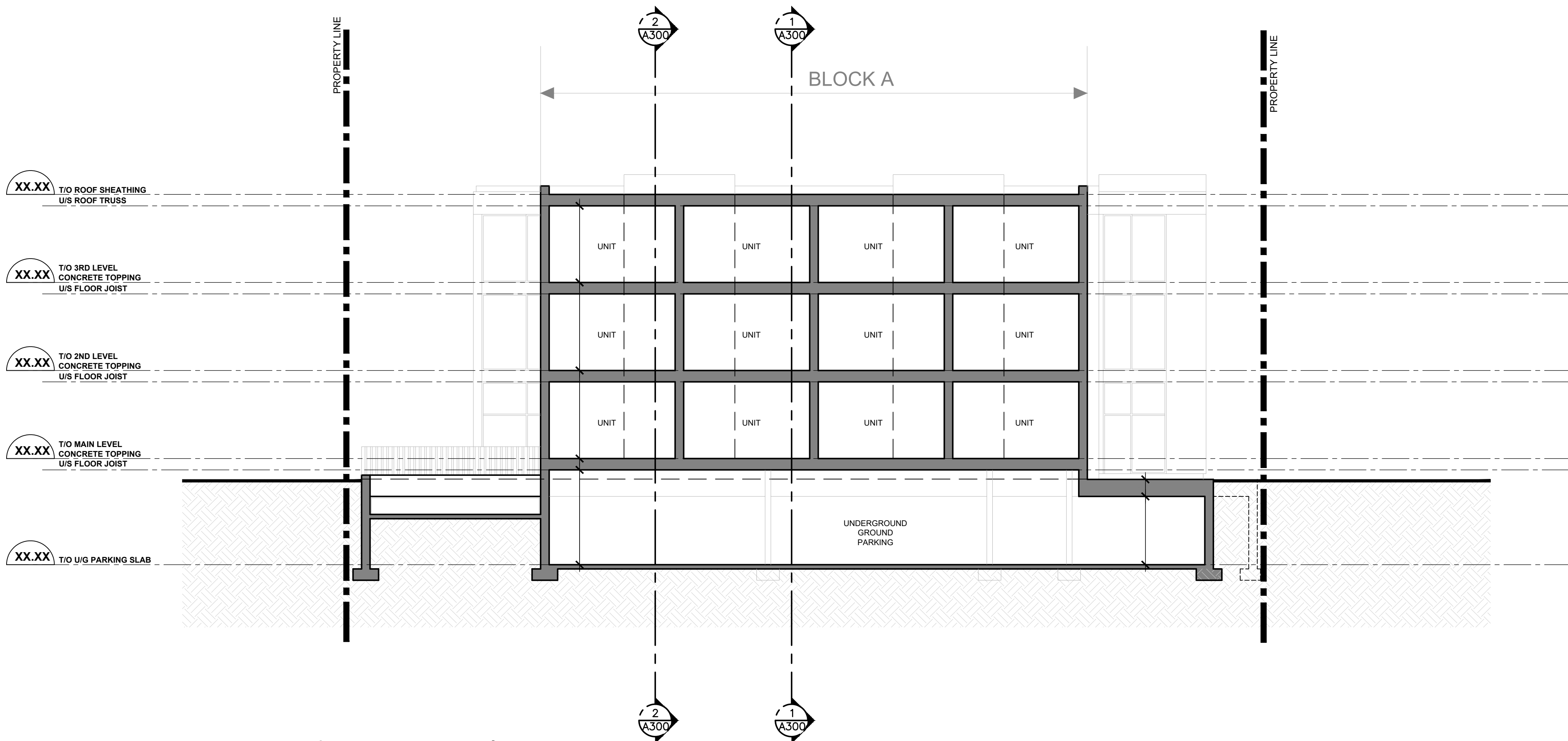
2 A-301 BUILDING_A SECTION (LOOKING WEST) SCALE = 1:100
