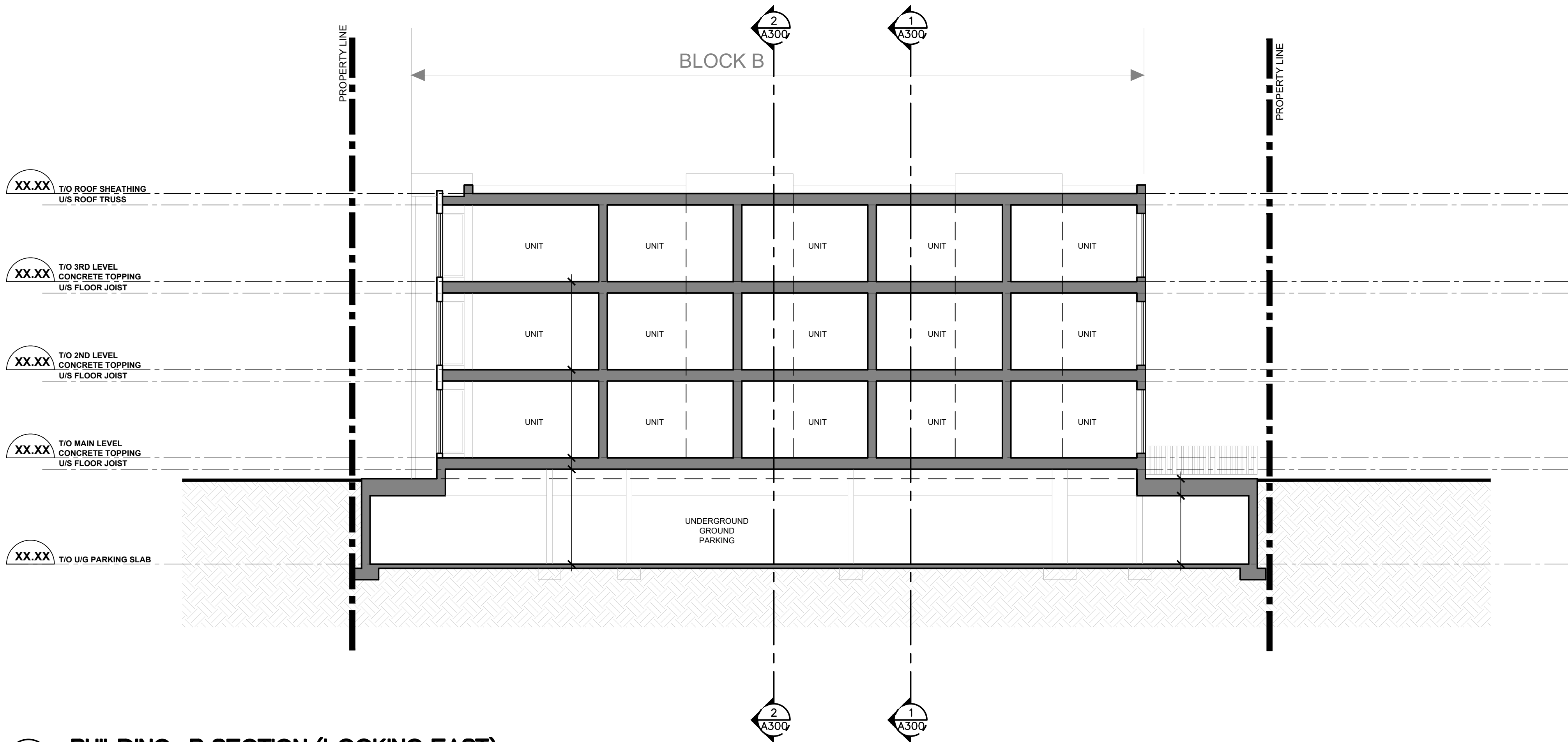
1 A-301 BUILDING_B SECTION (LOOKING EAST) SCALE = 1:100
