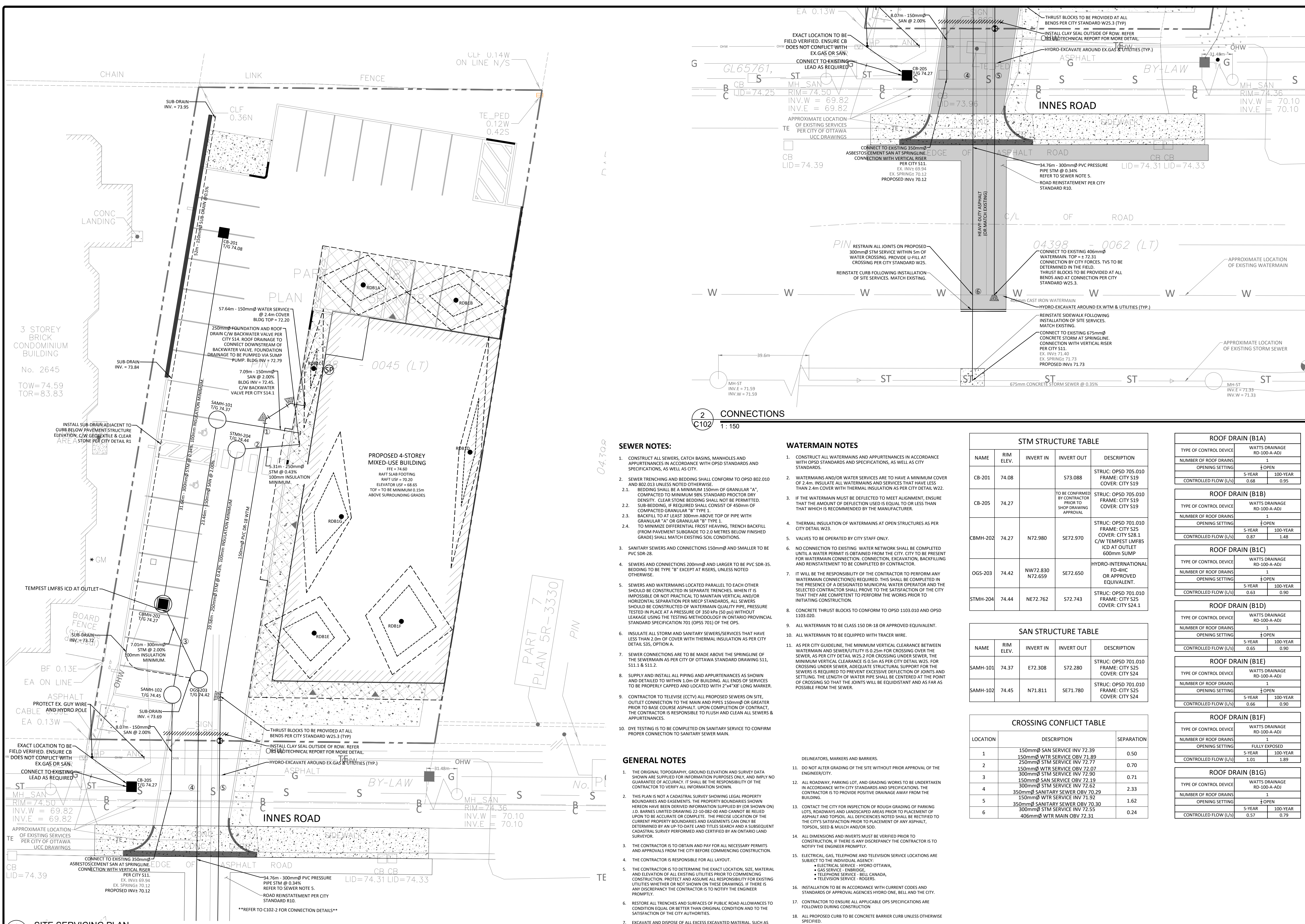
1 SITE SERVICING PLAN T: 150
