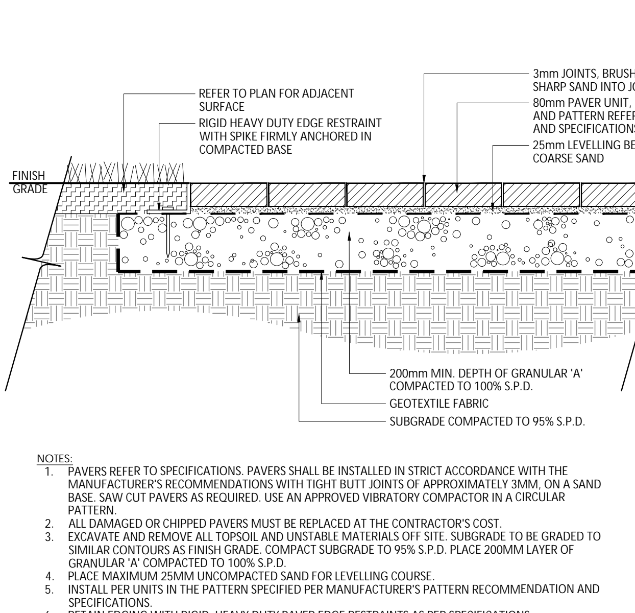
2 VEHICULAR UNIT PAVING N.T.S.
